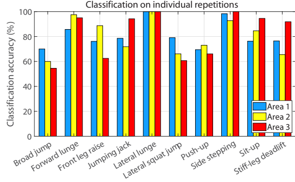
Fig. 9. Classification accuracy for each activity class in each test area, when using individual repetitions.
