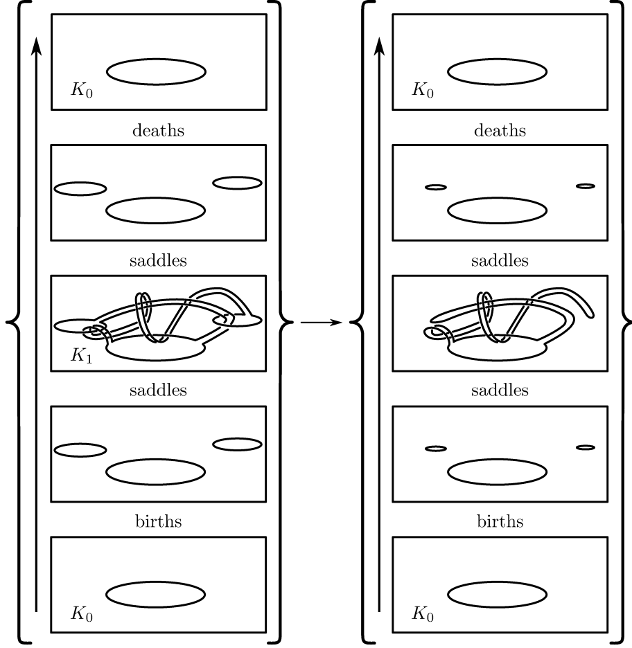
FIGURE 3.1. The modification of C' \circ C from the proof of Theorem 1.1. On the left is C' \circ C . On the right is the concordance obtained by replacing the disks D'_i with D_i . The concordance on the right is isotopic to [0, 1] \times K_0 .
