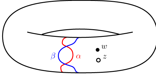
FIGURE 3.2. A diagram for the unknot \mathbb{O} in S^1 \times S^2 . The two intersection points both represent the torsion \text{Spin}^c structure.
