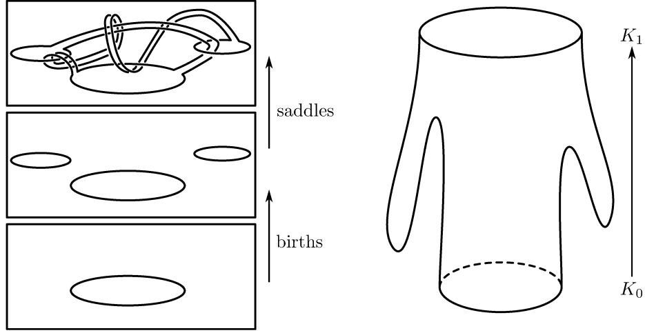
FIGURE 1.1. A ribbon concordance from K_0 to K_1 .
