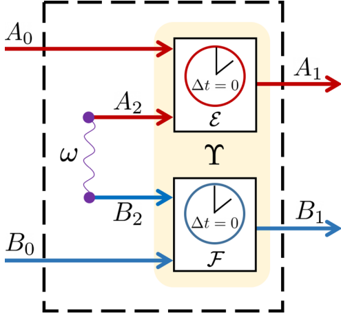
FIG. 9. Implementation of an LOSE quantum process with an entangled state \omega \in \mathfrak{D}(A_2 B_2) and local superprocess \Upsilon that takes the quantum state \omega^{A_2 B_2} as its input and then outputs the bipartite quantum channel \mathcal{N}^{AB} := \Upsilon[\omega^{A_2 B_2}] .
