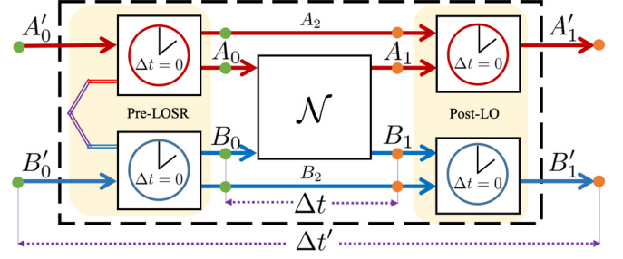
FIG. 10. An LOSR superprocess with \Delta t = \Delta t' .
