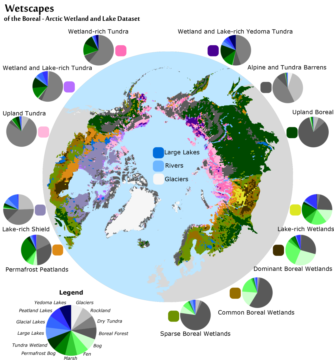
Figure 6. Wetscapes of the Boreal–Arctic Wetland and Lake Dataset. Wetscapes are defined by their characteristic composition of the BAWLD land cover classes and thus group regions with similar abundances (or absences) of specific wetland, lake, and river classes. The 15 wetscapes have their average land cover composition indicated by pie charts, with the legend shown in the bottom left. For clarity, the small and mid-sized lake classes were combined for glacial, peatland, and yedoma lakes, and the river classes were omitted from the pie charts. No land cover pie charts are shown for the Large Lakes, Rivers, and Glaciers wetscapes.
