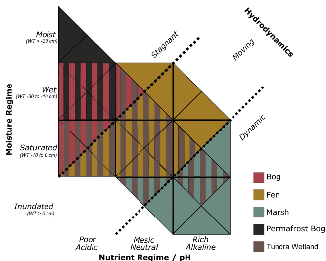
Figure 1. Descriptions of wetland classes in BAWLD as distinguished based on the moisture regime, the nutrient and pH regime, hydrodynamics, and the presence/absence of permafrost.
