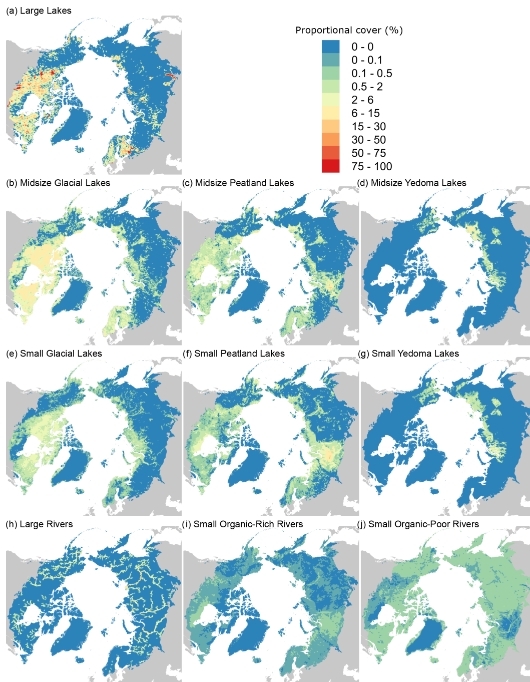
Figure 5. Predicted distributions of lake and river classes within the BAWLD domain: (a) Large Lakes, (b) Midsize Glacial Lakes, (c) Midsize Peatland Lakes, (d) Midsize Yedoma Lakes, (e) Small Glacial Lakes, (f) Small Peatland Lakes, (g) Small Yedoma Lakes, (h) Large Rivers, (i) Small Organic-Rich Rivers, (j) Small Organic-Poor Rivers.
