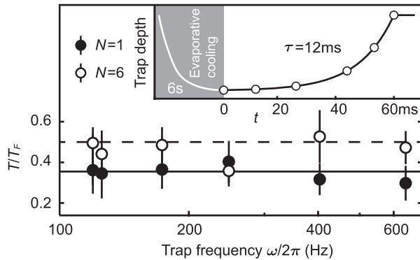
FIG. 6. The ramp-up of the optical dipole trap. T/T_F of both noninteracting gases ( N = 1 ) and weakly interacting gases ( N = 6 ) are conserved during ramping up the optical dipole trap. The ODT is increased exponentially in t_{\text{ramp}} = 60 ms with the time constant \tau = 12 ms (inset). Gases with N = 1 and N = 6 components are initially prepared at T = 0.35T_F and 0.5T_F , respectively.
