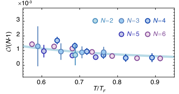
FIG. 8. Scaled contact vs temperature. Contact of different SU( N ) gases is scaled on the N = 2 components case by C/(N - 1) . The solid curve is the theoretical simulation multiplied by a factor of 7.5.
