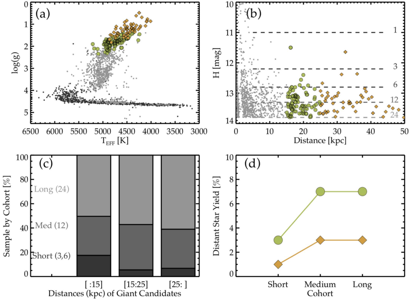
Figure 2. Evaluation of the Washington+DDO51 giant preselection in the APOGEE-2N Main Survey halo program for distant halo stars (e.g., PROGRAMNAME=“halo” and TELESCOPE=“apo25m”). (a) Spectroscopic \log g vs. T_{\text{eff}} for APOGEE-observed giant candidates (gray) and dwarf candidates (black) demonstrating the overall effectiveness of the Washington + DDO51 preselection technique. Stars with distances between 15 and 25 kpc are shown as green circles, and those with distances greater than 25 kpc as yellow diamonds. (b) Spectrophotometric distance against apparent H magnitude for giant candidates (gray) and the distant star samples (green and yellow). Horizontal dashed lines indicate the magnitude limits for targeting at the specified number of visits (labeled on the right). (c) After separating the giant candidate sample into distance bins ( d < 15 kpc, 15 < d < 25 kpc, 25 < d ), the fraction of the sample identified in the long (24-visit), medium (12-visit), and short (3- or 6-visit) “cohorts” on the plate designs. (d) The yield of distant stars within each “cohort” defined as N_{\text{distant}}/N_{\text{total}} , with N_{\text{total}} being the number of giant candidates.
