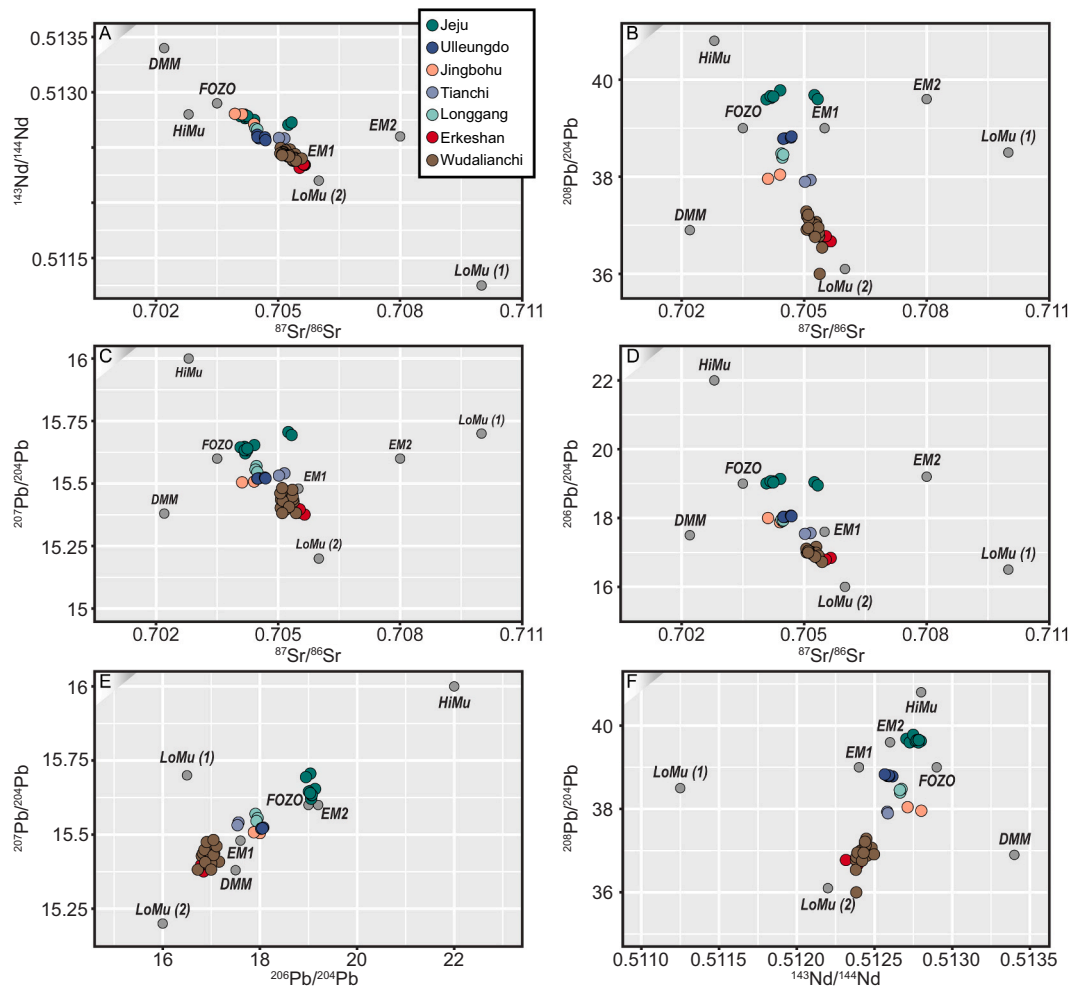
Fig. 12. Bivariate plots of key isotope data from intraplate volcanoes in East Asia. Samples of all \text{SiO}_2 concentration are shown in these plots. Jeju displays the most radiogenic isotope compositions. Erkeshan and Wudalianchi are noteworthy for displaying very low ^{208}\text{Pb}/^{204}\text{Pb} , ^{207}\text{Pb}/^{204}\text{Pb} and ^{206}\text{Pb}/^{204}\text{Pb} values. The remaining intraplate volcanoes usually plot between the radiogenic values of Jeju and the unradiogenic values of Erkeshan and Wudalianchi. Data sources are listed in Supplementary Table S1. Isotope reservoir values are from Chen et al. (2007) and authors therein.
