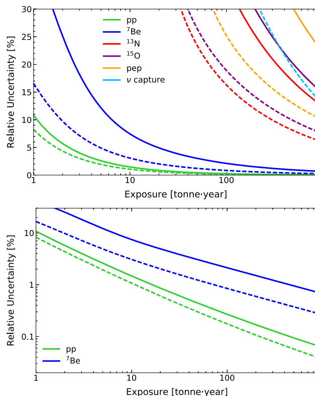
Fig. 2 The measured relative uncertainty of each solar neutrino component and neutrino capture as a function of exposure. The median fluxes of the high- Z model are assumed. Solid (dashed) curves correspond to a natural (depleted) target. A log scale of the pp and ^7\text{Be} components is shown in the bottom panel for clarity
