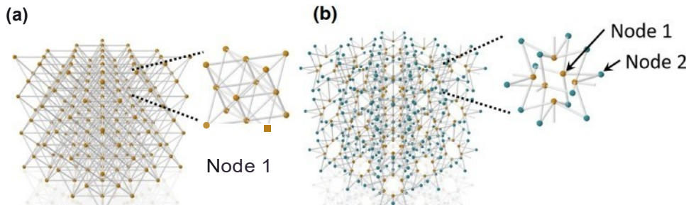
FIG. 6. (a) Identical nodes in a conventional octet-truss lattice [19,42]. (b) The two different nodes of the isotoxal auxetic unit cell that is proposed here.
