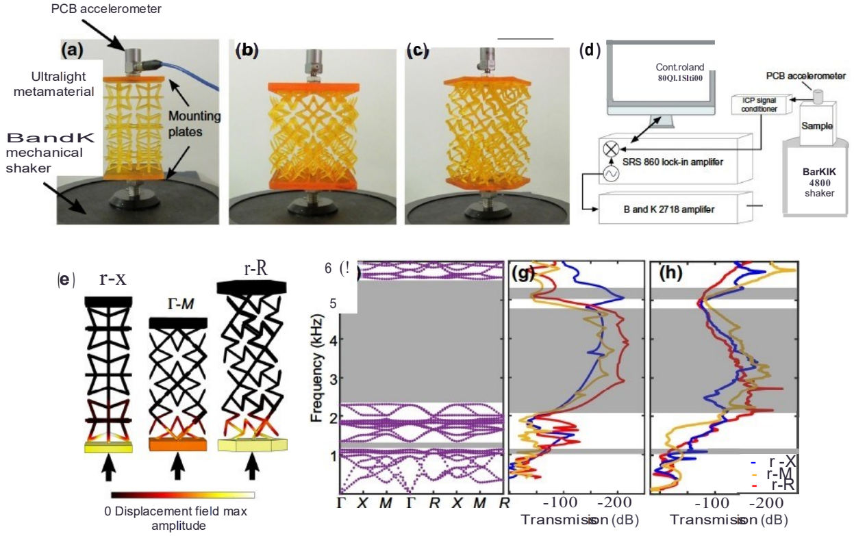
FIG. 4. Photograph of the measurement platform with the (a) r -X, (b) r -M, and (c) r -R samples mounted, (d) schematic of the experimental measurement setup, (e) numerical results of the normalized displacement field for the \Gamma -X, \Gamma -M, and \Gamma -R samples, for a frequency of excitation of 4 kHz, (f) band structure (in kHz), for the unit cell, where \mu = 20^\circ , d = 0.06p , and a = 0.8p , and the material properties are E = 512 MPa, \nu = 0.3 , and \rho = 1.1 g/cm 3 . (g) Results from frequency-domain transmission simulations through the three samples under consideration with \mu = 21^\circ , corrected material properties (shown in Fig. 10 in Appendix F) and an isotropic loss factor of 0.01. (h) Experimentally measured elastic wave transmission (dB) through the r -X, r -M, and r -R samples denoted by the blue, orange, and red curves, respectively. The shaded gray regions in (f)-(h), indicate the BGs.
