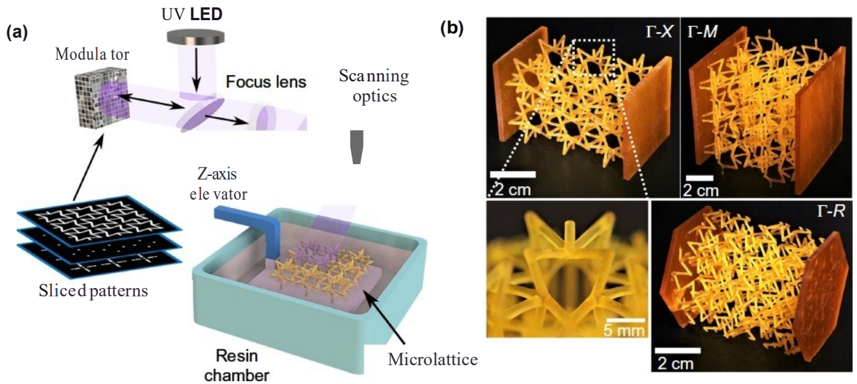
FIG. 9. (a) Schematic illustration of the fabrication technique. (b) Photographs of the ultralight isotoxal star-based metamaterial samples, fabricated in the \Gamma-X (top left), \Gamma-M (top right), and \Gamma-R (bottom right) directions, with the same unit-cell dimensions and with period, p = 2 cm. Bottom left shows a close-up optical image of the \Gamma-X sample, featuring the overhanging structure in the present metamaterial.
