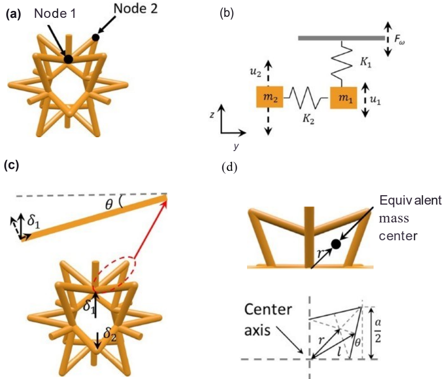
FIG. 7. (a) Unit cell of the proposed 3D elastic metamaterial with the two nodes described in Appendix B, (b) shows its equivalent spring-mass system. F_w is the external excitation, while u_1 and u_2 denote the displacements of the individual masses. (c) The bottom shows the isotoxal auxetic unit cell that experiences the displacements, \delta_1 and \delta_2 at nodes 1 and 2, respectively. The top shows node 1 attached to an inclined strut, with an angle, \theta . (d) The top shows the equivalent mass center for node 2 that is offset from the center axis and the bottom indicates the parameters, r , l , and \theta , in this context.
