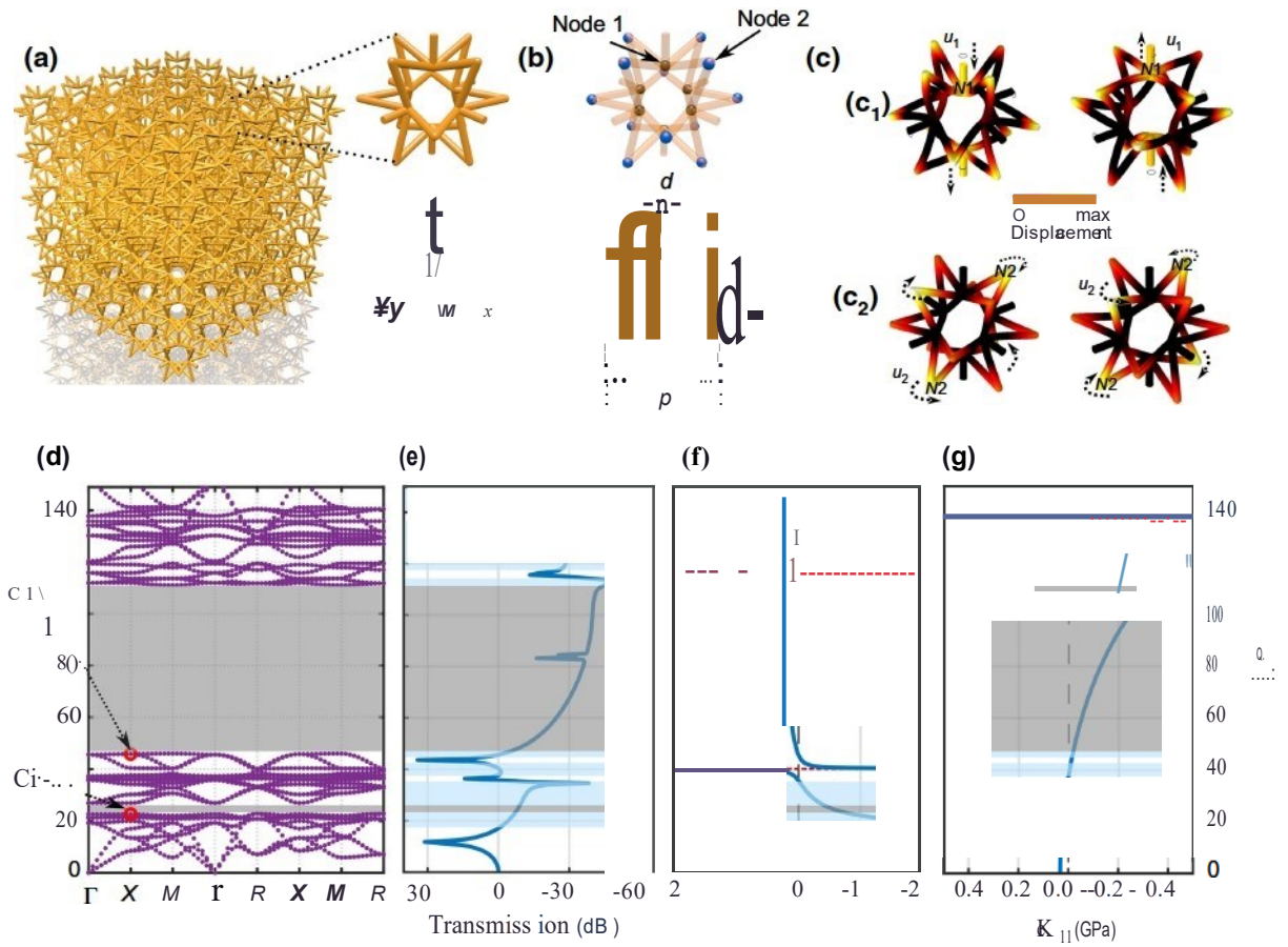
FIG. 1. (a) Ultralight microlattice-based elastic metamaterial composed of periodic auxetic building blocks (top right) and the directions of the irreducible Brillouinzone, for the simple cubic unit cell (bottom right). (b) (Top) Nodes 1 and 2 of the unit cell, denoted by the black and blue spheres, respectively. (Bottom) Dimensions of the unit cell: p is the periodicity, and a is the distance between the vertices of the isotoxal squares, \beta is the angle between the outer edges of the isotoxal square stars and the vertical. (c) Snapshots of the resonance modes that give rise to bandgaps. u_1 and u_2 denote the longitudinal and torsional displacement of the nodes 1 (N1) and 2 (N2), respectively. (d) Normalized band structure for the simple cubic auxetic unit cell along the different directions of the IBZ, for \beta = 20^\circ , a = 0.8p , and d = 0.060p . (c1) and (c2) are the modes at the X point (red circles) on the lower edges of the BGs. (e) Longitudinal wave transmission in dB, for propagation in the r - X direction. Frequency dependent (f) effective density, \rho_{\text{eff}} , and (g) effective bulk modulus, \kappa_{\text{eff}} . The dashed red lines in (f) and (g) indicate sudden jumps in \rho_{\text{eff}} and \kappa_{\text{eff}} , from positive to negative values and vice versa. The regions in gray denote complete BGs, while those shaded blue indicate the BGs associated with longitudinal waves only.
