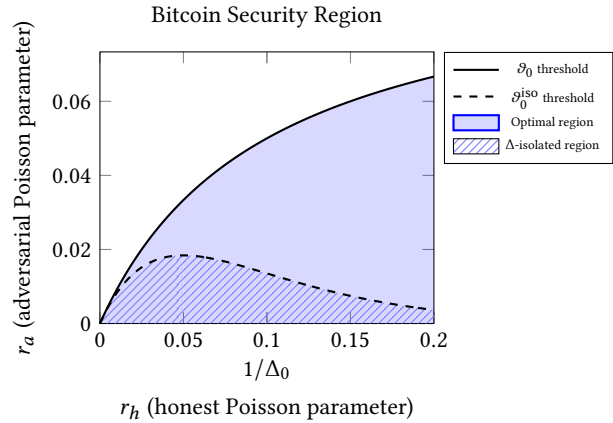
Figure 1: The region of pairs (r_a, r_h) for which Bitcoin is secure with \Delta_0 = 10 . The optimal bound established in this paper \vartheta_0 = 1/(\Delta_0 + 1/r_h) is shown in solid black; the region beneath this line—filled in light blue—is the region of pairs (r_a, r_h) for which we establish security. The best prior bound \vartheta_0^{\text{iso}} = r_h \exp(-2\Delta_0 r_h) is shown in dashed black; its corresponding region of security is shown with blue hatching.
