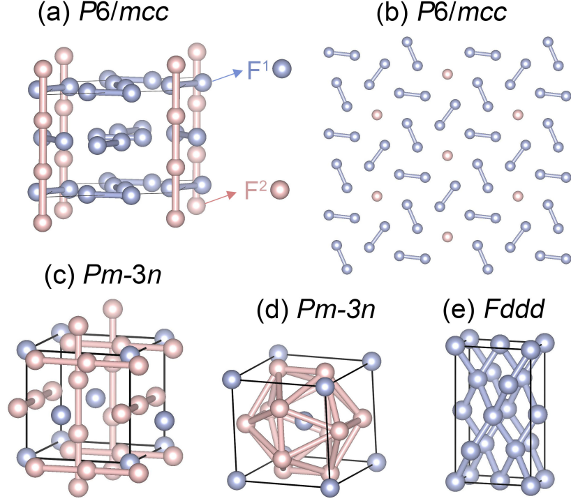
FIG. 2. (color online). Crystal structure of fluorine phases. (a) The crystal structure of P6/mcc . The F^1 and F^2 are shown using blue and pink spheres, respectively. (b) A layer of the P6/mcc structure. The layers are stacked in an ABCBA fashion. (c) The crystal structure of Pm\bar{3}n showing polymeric line chains. (d) The crystal structure of Pm\bar{3}n showing icosahedron. (e) The crystal structure of atomic phase Fddd .
