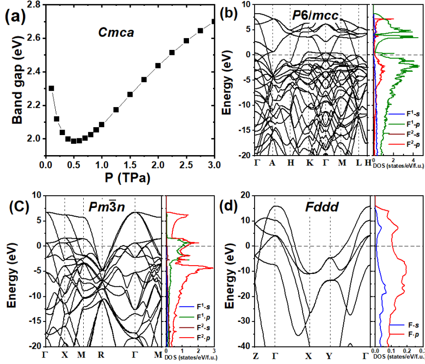
FIG. 4. (color online) (a) Variation of band gaps with pressure for Cmca . Band structure and partial densities of states (PDOS) of (b) P6/mcc phase at 3 TPa, (c) Pm3n Phase at 5 TPa, (d) Fddd at 30 TPa.
