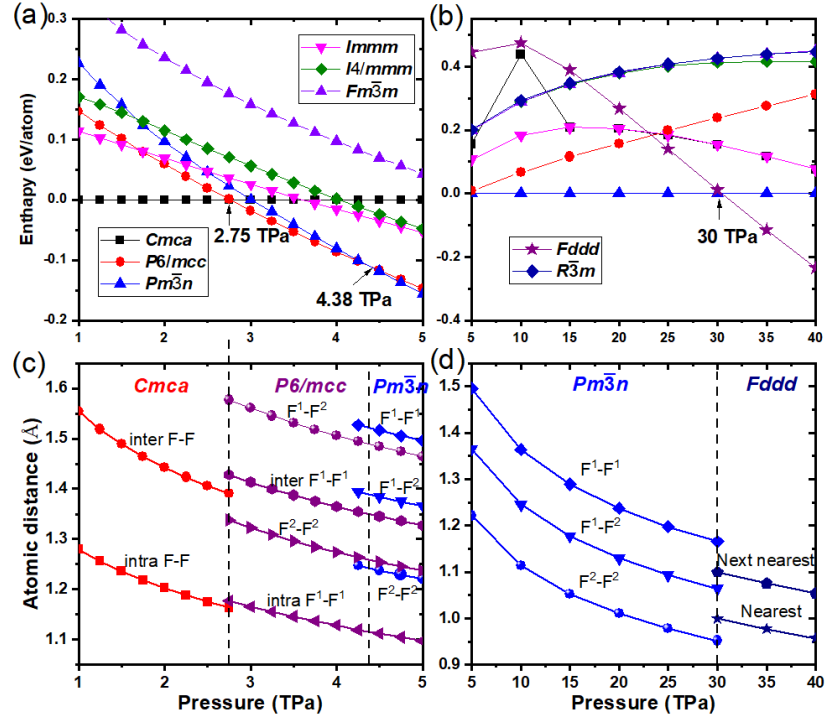
FIG. 1. (color online). Enthalpy difference curves of various structures relative to (a) the Cmca structure below 5 TPa and (b) the Pm3n structure between 5-40 TPa. (c) and (d) The nearest F-F distances (intra F-F) and the next nearest F-F distances (inter F-F) in the Cmca phase; the nearest F 1 -F 1 distance (intra F 1 -F 1 ), the next nearest F 1 -F 1 distance (inter F 1 -F 1 ), the nearest F 2 -F 2 distance (F 2 -F 2 ), and the neighboring F 1 -F 2 distance (F 1 -F 2 ) in P6/mcc phase; the nearest F 2 -F 2 distance (F 2 -F 2 ), the nearest F 1 -F 1 distance (F 1 -F 1 ), the neighboring F 1 -F 2 distance (F 1 -F 2 ) in Pm3n phase, the nearest and next nearest F-F distance in Fddd phase as function of pressure.
