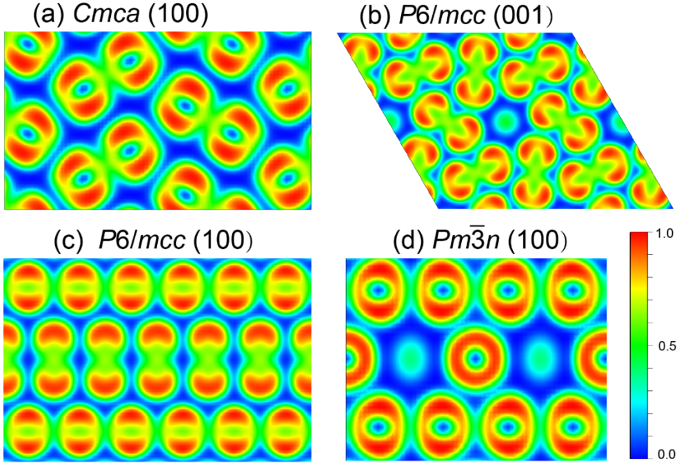
FIG. 3. The calculated ELF of our predicted phase. (a) Cmca in the (100) section at 3 TPa. (b) and (c) P6/mcc in the (001) and (100) section at 3 TPa. (d) Pm\bar{3}n in the (100 section) at 5 TPa.
