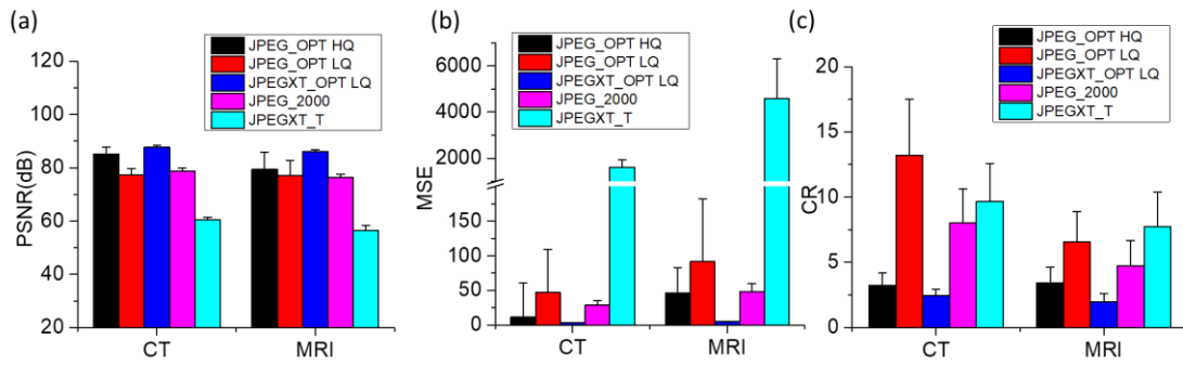
Figure. 8 Evaluation of ROI_REGN_EDG-based compression of CT and MRI images by using JPEG_OPT HQ and JPEG_OPTLQ, JPEGXT_OPT LQ, and the traditional methods: JPEGXT_T and JPEG_2000. (a) PSNR; (b) MSE; (c) CR. LQ compression of JPEG_OPT: CT: N=10, NDP=1; MRI: N=50, NDP=1.
