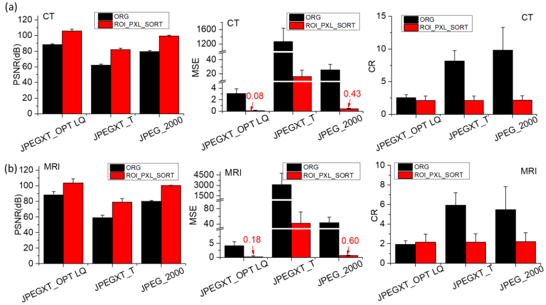
Figure. 6 Evaluation of the ORG and ROI_PXL_SORT compression of CT and MRI images by using JPEGXT_OPT LQ, and the traditional methods: JPEGXT_T, and JPEG_2000. (a) PSNR, MSE, and CR in CT; (b) PSNR, MSE, and CR in MRI.
