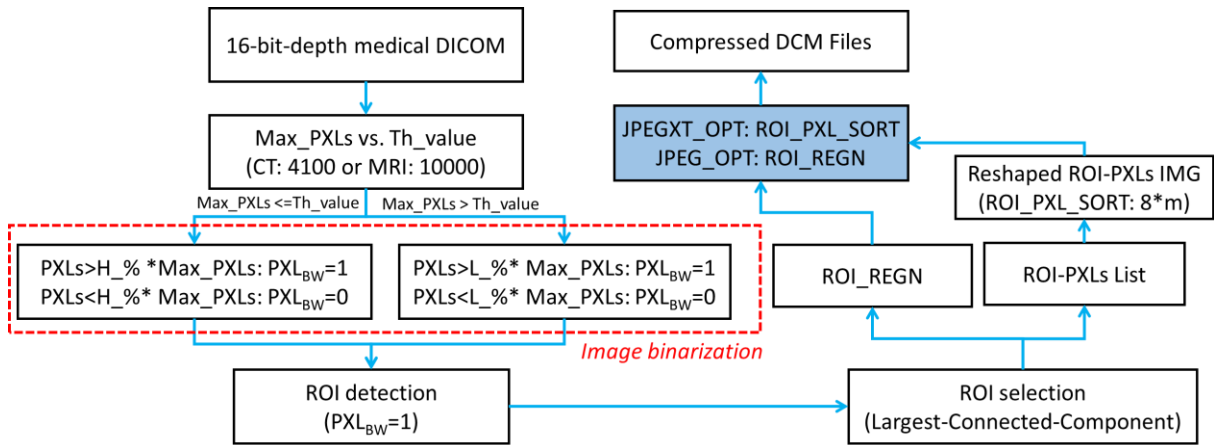
Figure. 1 The flowchart of ROI-based JPEGXT_OPT algorithm for the compression of 16-bit depth medical images.
