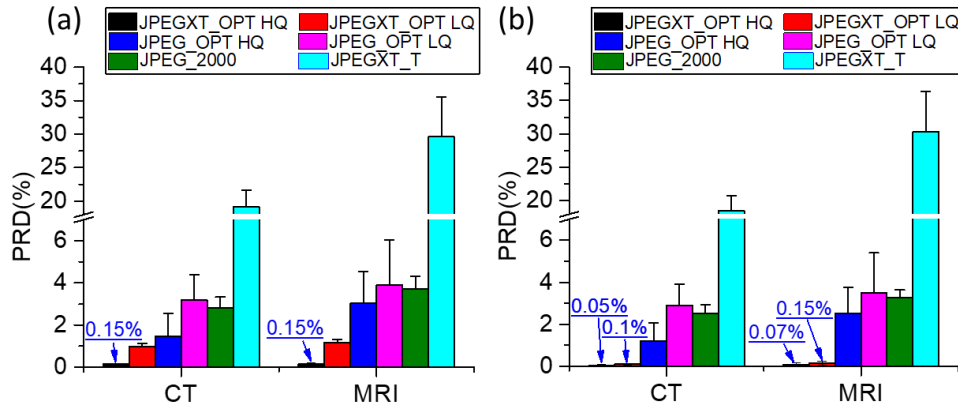
Figure. 11 PDR of CT and MRI compression under different JPEG-based approaches. (a) ORG; (b) ROI_PXL-SORT (JPEGXT_OPT) and ROI_REGN_EDG (JPEG_OPT, JPEGXT_T and JPEG_2000).
