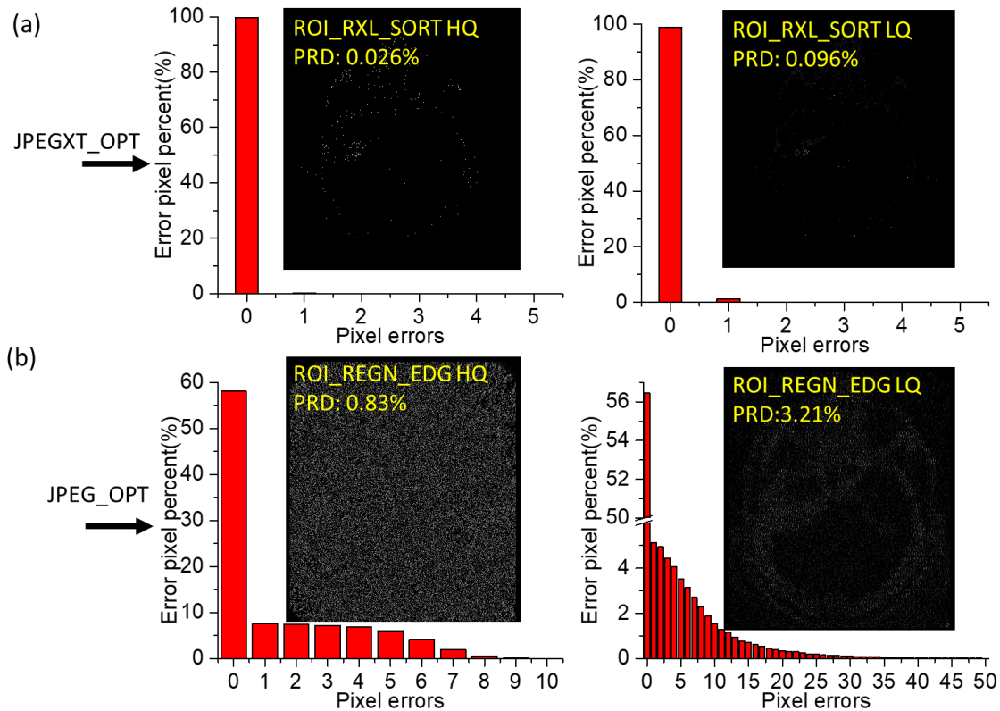
Figure. 12 Prediction error images and their corresponding histogram of the CT image compressed by ROI-based JPEGXT_OPT and JPEG_OPT approaches. (a) JPEGXT_OPT with high and low-quality ROI_PXL_SORT; (b) JPEG_OPT with high and low-quality ROI_REGN_EDG.
