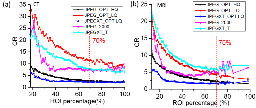
Figure. 9 CR distributions under different ROI percentages by using the ROI_REGN_EDG method under JPEG_OPT, JPEGXT_OPT, and compared to the traditional methods: JPEGXT_T, and JPEG_2000. (a) CT; (b) MRI.
