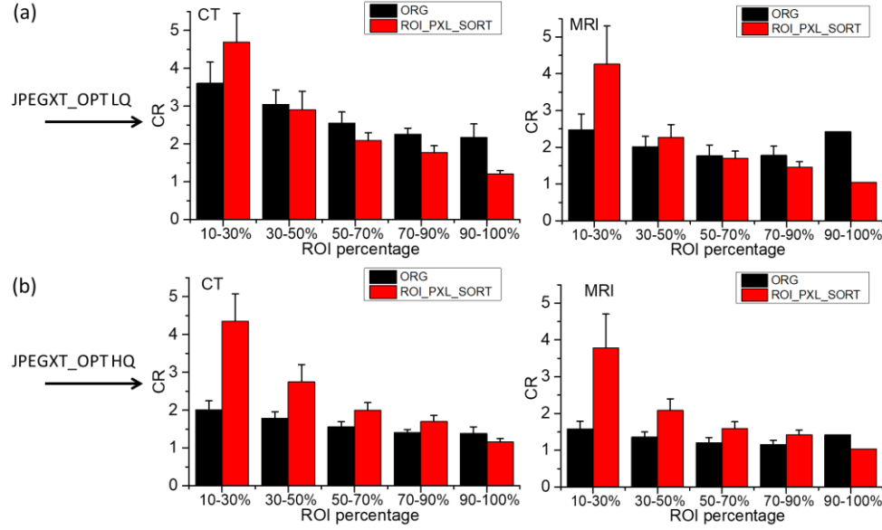
Figure. 5 CR distributions under different ROI percentages between ORG compression and ROI_PXL_SORT by using JPEGXT_OPT. (a) JPEGXT_OPT LQ; (b) JPEGXT_OPT HQ.
