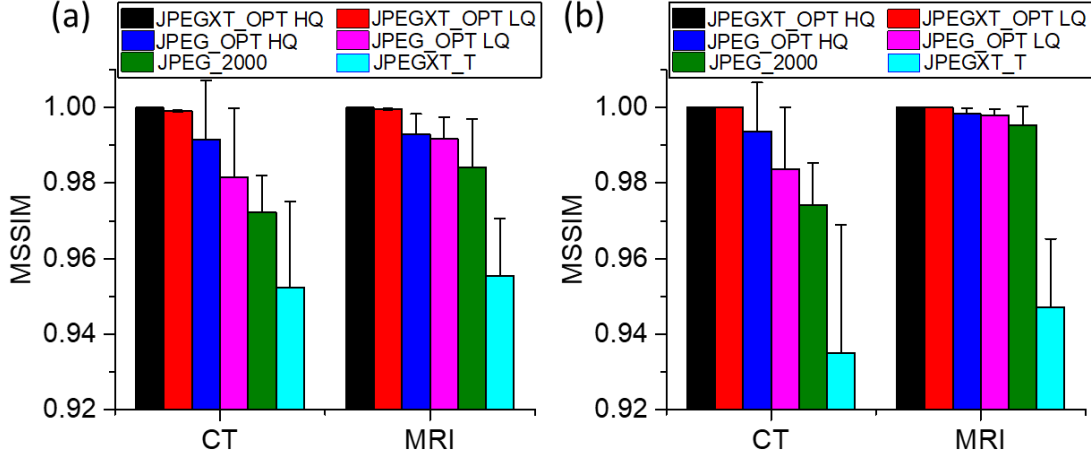
Figure. 10 MSSIM of CT and MRI compression under different JPEG-based approaches. (a) ORG; (b) ROI_PXL-SORT (JPEGXT_OPT) and ROI_REGN_EDG (JPEG_OPT, JPEGXT_T and JPEG_2000).
