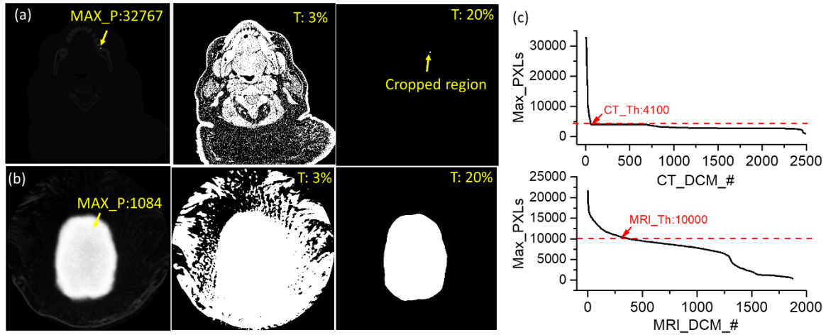
Figure. 2 ROI region detection based on the thresholds of the maximum pixels. (a) ROI detection in large maximum pixel values; (b) ROI detection in small maximum pixel values; (c) The maximum pixel distributions in the CT and MRI images.
