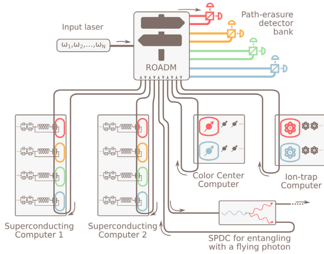
FIG. 3. Future outlook for interfidge connectivity. Replacing the single path-erasure detection with a reconfigurable optical add-drop multiplexer (ROADM) will allow us to route a frequency comb pump laser to qubits in several quantum nodes. By connecting the ROADM to a bank of path-erasure detectors for each frequency channel, this design will enable multiplexed heralded entanglement generation between multiple fridges of different quantum modalities.
