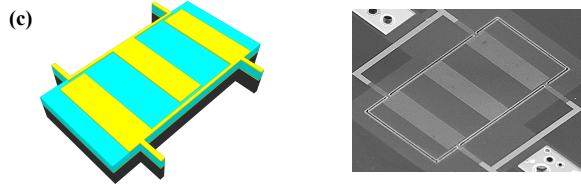
Figure 1. (a) Schematic diagram (left) and Scanning Electron Microscopy (SEM) micrograph (right) of 85% top electrode coverage. (b) Schematic diagram (left) and Scanning Electron Microscopy (SEM) micrograph of 60% top electrode coverage. (c) Schematic diagram (left) and Scanning Electron Microscopy (SEM) micrograph of 40% top electrode coverage.
