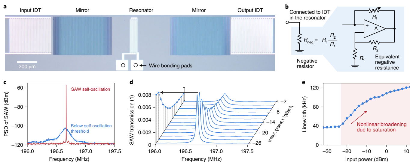
Fig. 2 | Characterization of SAW gain and nonlinearity. a , Microscope image of a single SAW resonator for gain and nonlinearity characterization. The gain for the SAWs is provided by the interdigital electrodes connected to an electronic circuit by wire bonding. b , Electronic diagrams of the negative resistor providing SAW gain. The negative resistance is implemented by an operational amplifier and resistors. The equivalent negative resistance is tuned using the adjustable resistor R_f . c , Measured power spectral density (PSD) of the output SAW from the active resonator. When the gain is below the threshold for self-oscillation, the spectrum of the SAW collected at the output IDT shows resonance with a linewidth of 94(1) kHz determined by the quality factor of the resonator ( Q=2,000 ). When the gain is increased above the threshold, the resonator linewidth narrows below 2.5 kHz (the spectral resolution set by the spectrum analyser) and SAW self-oscillation is observed. d,e , Transmission spectra ( d ) and linewidth ( e ) of the nonlinear active resonator for various SAW input powers. The transmission resonance broadens, and its amplitude reduces for greater input powers due to the nonlinear saturation.
