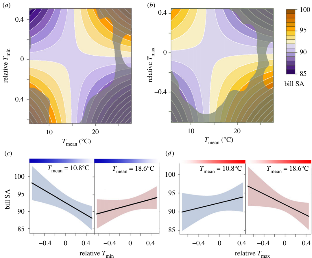
Figure 2. The relationship of bill surface area (purple-to-orange gradient, in \text{mm}^2 ) with relative minimum temperature (a) and relative maximum temperature (b) varied depending on the 5-year mean temperature, but in opposite directions. Contour plot area outside of the kernel density space containing 99.9% of datapoints is shaded grey. (c) Relative minimum temperature (blue gradient, with darker shades indicating more unusually cool temperatures) was positively associated with bill surface area when the mean temperature was high (confidence interval in pink), but negatively associated when the mean temperature was low (confidence interval in blue); the temperatures shown, 10.8 and 18.6^{\circ}\text{C} , are the 10th and 90th percentiles of mean temperature. (d) Relative maximum temperature (red gradient, with darker shades indicating more unusually warm temperatures) exhibited the opposite relationship with bill surface area with regards to mean temperature.
