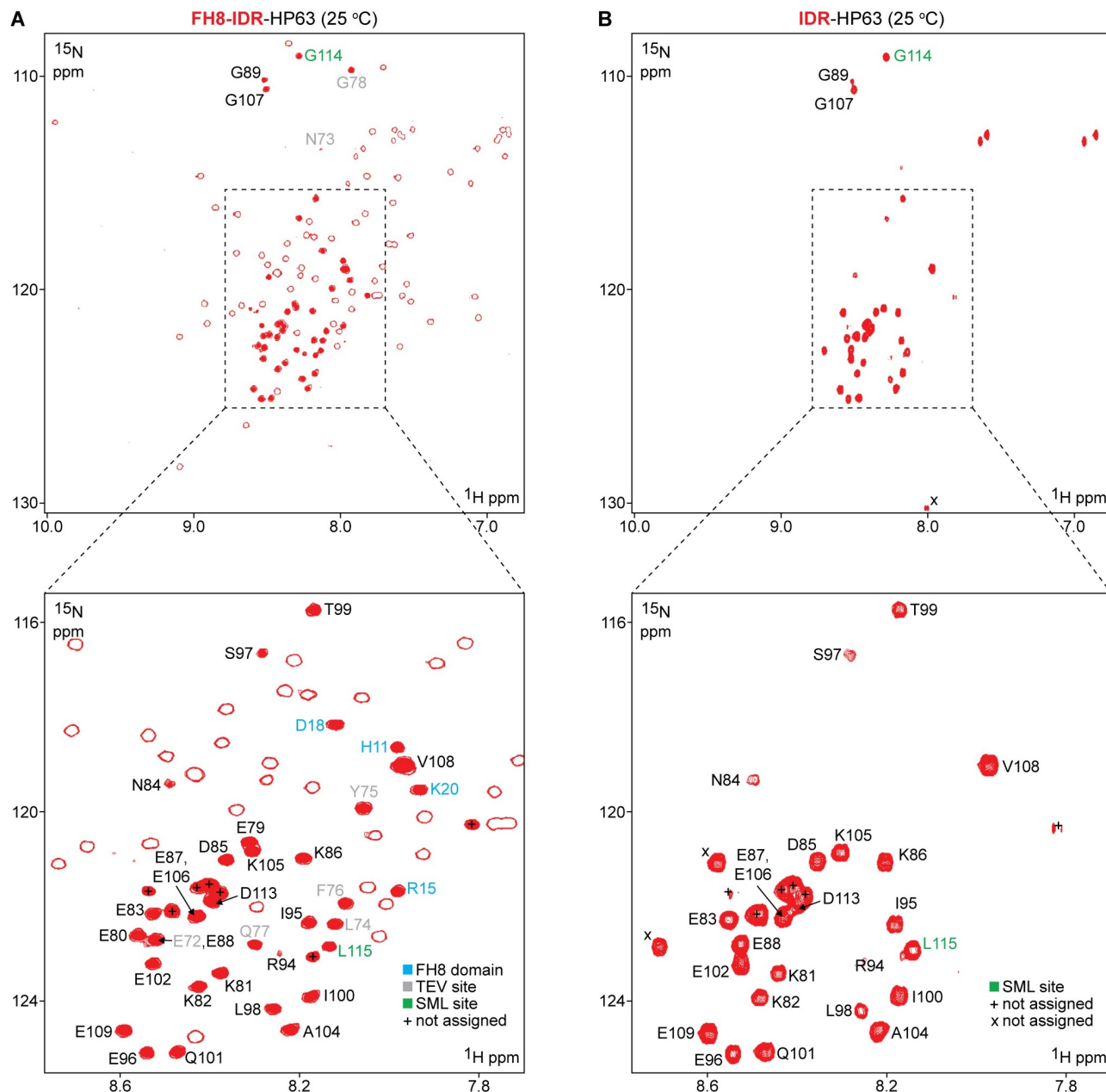
Fig 5. ^{15}\text{N} -HSQC NMR spectra (25°C) of segmentally labeled FH8-IDR-HP63 and IDR-HP63. (A) Spectrum recorded at 600 MHz ( ^1\text{H} frequency) with 256 indirect increments using a FH8-IDR-HP63 sample with the FH8-IDR portion segmentally labeled with ^{13}\text{C}/^{15}\text{N} isotopes. All observed resonances for the labeled FH8-IDR segment are represented by open red contours, and signals that have been segmentally assigned to the IDR linker portion are overlaid with solid red ovals. Residue-specific NMR assignments for 36 residues in the linker region (27 from the villin 4 IDR and 9 residues from the flanking TEV and sortase ligation sites) and four FH8 domain peaks (false positives from the segmental assignment) are indicated with residue numbers. The numbers for the TEV site (7 residues) are shown in grey, FH8 domain (4 residues) are shown in blue, and two residues corresponding to the SML ligation site (G114, L115) are shown in green. Seven segmentally assigned peaks for which no residue specific assignments were obtained are marked with "+". Residue numbers shown correspond to the sequence of FH8-IDR-HP63 (see S2 Fig). To relate the assigned IDR residues to the corresponding positions in wild type villin 4, a value of 798 should be added. (B) Spectrum recorded at 500 MHz ( ^1\text{H} frequency) with 196 indirect increments using an IDR-HP63 sample with the IDR segmentally labeled with ^{15}\text{N} isotopes. All observed resonances for the labeled IDR segment are represented by solid red signals. Residue-specific NMR assignments for 25 residues in the linker region were unambiguously transferred from panel A (out of 27 listed on panel A). Three new resonances were observed (marked with "x") following removal of FH8. Two of these are presumed to correspond to residues E79 and E80, which are adjacent to the newly formed N-terminal residue G78. The two residues corresponding to the SML ligation site (G114, L115) are shown in green. As in the case of FH8-IDR-HP63 (panel A), additional peaks (6 total) for which no residue specific assignments were obtained are marked with "+".
