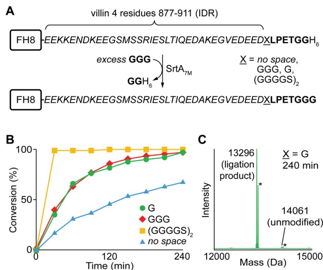
Fig 3. Effect of linker structure on SML using villin 4 IDR substrates. (A) Model SML reaction for comparing ligation efficiency with IDR substrates containing different spacers. (B) Time course demonstrating improved ligation efficiency when spacers were included between the IDR and LPXTG motif. Reaction progress was estimated using LC-ESI-MS. (C) ESI-MS spectrum of SML reaction mixture for the substrate containing a single glycine (G) spacer following a 4 h incubation at room temperature (calculated MWs: unmodified substrate = 14062 Da, ligation product = 13296 Da, * = MeCN adducts from LC-ESI-MS mobile phase).
