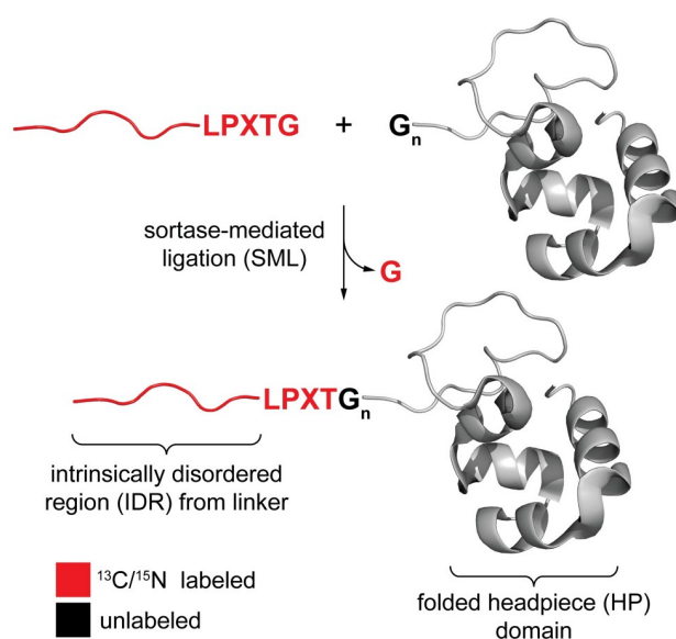
Fig 1. Segmental isotopic labeling via Sortase-Mediated Ligation (SML). Strategy for segmental isotopic labeling of villin 4 utilizing SML between the disordered linker and folded headpiece. LPXTG represents the requisite sortase recognition site.
