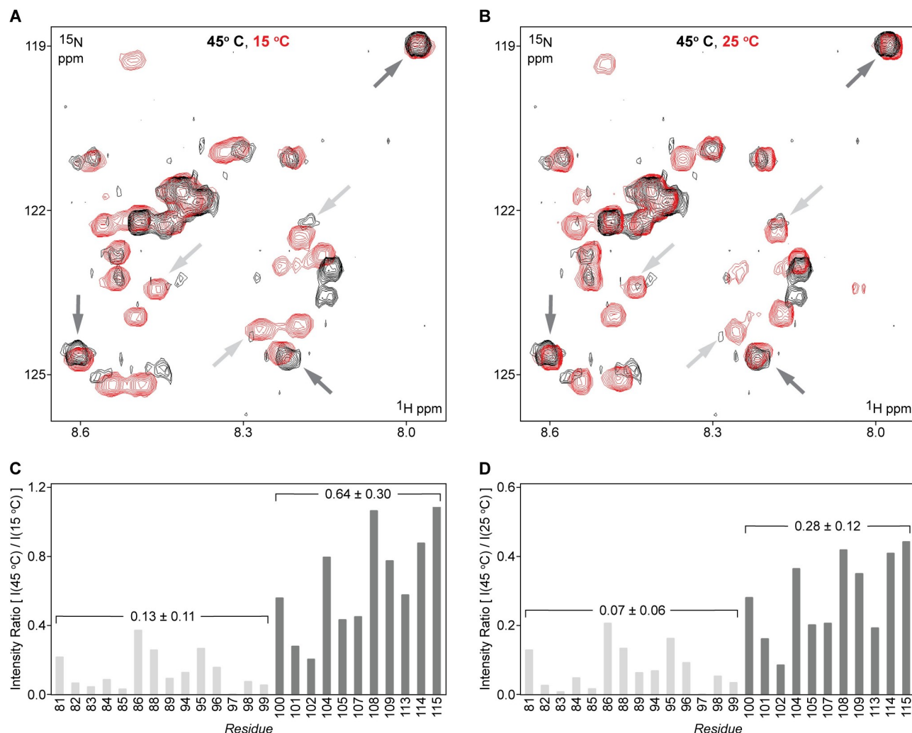
Fig 6. Temperature sensitivity in the 35-residue acidic segment of the villin 4 IDR. Representative regions of ^{15}\text{N} -HSQC NMR spectra (500 MHz, ^1\text{H} frequency) for IDR-HP63 with the IDR segmentally labeled with ^{15}\text{N} isotopes recorded at (A) 45°C (black) / 15°C (red) and (B) 45°C (black) / 25°C (red). Spectra recorded at 15°C and 45°C were re-referenced to the ^1\text{H} / \text{H}_2\text{O} chemical shift value (4.78 ppm) of the spectrum recorded at 25°C according to a standard approach [63]. The number of scans for the three spectra were 64 (15°C), 128 (25°C), and 192 (45°C), with 196 indirect increments ( ^{15}\text{N} dimension) in all three cases. (C) Ratios of ^{15}\text{N} -HSQC backbone amide signal intensity for assigned IDR residues at 45°C and 15°C, and (D) a corresponding data set for signal intensity ratios at 45°C and 25°C. In both panels C and D, data points for residues 81–99 are colored in light grey, and dark grey for residues 100–115. Light grey and dark grey arrows on panels A and B point to select signals representing each of these two respective groups. Data points for residues 87 (from the light grey group) and 106 (dark grey group) are excluded from this analysis due to their resonance overlap. Values shown above the brackets represent the average intensity ratio ( \pm standard deviation) for the residues indicated.
