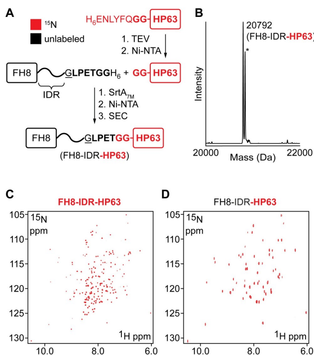
Fig 4. Segmental isotopic labeling of truncated villin 4. (A) SML strategy for producing segmentally labeled derivatives containing an IDR segment (35-residue acidic fragment) and the headpiece domain of villin 4. (B) ESI-MS spectrum of purified FH8-IDR-HP63 with selective incorporation of 15 N in the HP63 segment (calculated MW assuming 100% 15 N incorporation in HP63 = 20797 Da, * = MeCN adducts from LC-ESI-MS mobile phase). (C) 15 N-HSQC (500 MHz, 25°C) of uniformly labeled FH8-IDR-HP63. Based on the sequence of FH8-IDR-HP63, 176 resonances originating from non-proline residues are expected and 173 were observed. (D) 15 N-HSQC (500 MHz, 25°C) of segmentally labeled FH8-IDR-HP63 in which 15 N labeling is restricted to HP63. Based on the sequence of the labeled segment, 61 resonances originating from non-proline residues are expected and 58 were observed.
