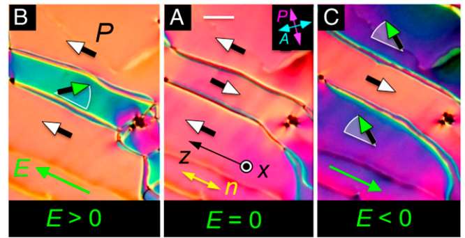
Fig. 2. DTLM images showing polar Fredericksz twist transition in ferroelectric domains with opposite polar orientation at T = 120^\circ\text{C} . These domains, grown field-free upon cooling from the N phase to this temperature, have a polarization density \mathbf{P} . (A) Field-free initial state showing three domains separated by domain walls, each domain having \mathbf{n}(\mathbf{r}) along the buffing direction z . (B) Application of an ultra-small, positive test field E_z = 1\text{ V/cm} induces a birefringence color change resulting from in-plane reorientation of \mathbf{n}(\mathbf{r}) in the center domain, leaving the upper and lower domains unchanged. (C) Application of E_z < 0 induces an in-plane reorientation of \mathbf{n}(\mathbf{r}) in the upper and lower domains. There is little optical change or reorientation in the central domain. If the field is returned to E = 0 , the system returns to the starting state (A). These observations demonstrate that the domains are polar and also enable the absolute determination of the direction of \mathbf{P}(\mathbf{r}) : domains that have the orientation preferred by the applied field do not reorient. In this experiment, \mathbf{P}(\mathbf{r}) and \mathbf{n}(\mathbf{r}) within the domains rotate about x but the field is not large enough to move the domain walls, which are pinned by the surfaces. The polarization vectors (shaded green) and circular arcs (white) depict the field-induced reorientation of \mathbf{P}(\mathbf{r}) in the midplane of the cell: \mathbf{P}(\mathbf{r}) does not reorient at the surfaces in this experiment, remaining parallel to the buffing direction. These field-induced reorientations with \mathbf{P}(\mathbf{r}) starting nearly antiparallel to \mathbf{E} are polar azimuthal Fredericksz transitions. The threshold field, E_P = (\pi/t)^2(K_{11}/P) , estimated using the measured P \sim 5\text{ }\mu\text{C/cm}^2 at T = 120^\circ\text{C} (Fig. 3), is E_P \sim 1\text{ V/cm} , comparable to the fields employed here. t = 11\text{ }\mu\text{m} . (Scale bar, 30\text{ }\mu\text{m} .)
