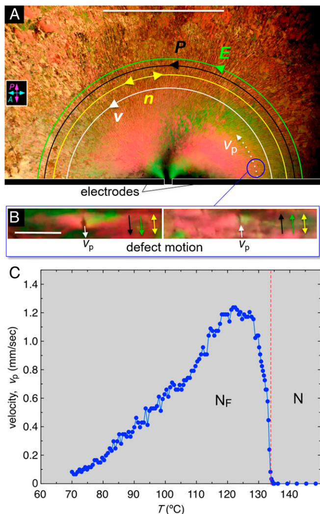
Fig. 6. Field-induced flow in the ferroelectric nematic phase. (A) DTLM image of a t = 10\text{-}\mu\text{m} -thick, planar-aligned cell of RM734 between untreated glass plates, in the N_F phase at T = 120^\circ\text{C} . The black bars at the bottom are two evaporated gold electrodes on one of the plates, separated by a d = 60\text{ }\mu\text{m} gap. The electrodes are outlined in white for clarity. Only the upper edges of the electrodes and the adjacent part of the cell are shown. A square-wave voltage with V_p = 3\text{ V} , 0.1\text{ Hz} , is applied to the electrodes, producing an electric field in the plane of the cell. This field drives a pattern of defect motion and fluid flow over the entire field of view, with the defect velocity \mathbf{v}(\mathbf{r}) (white arrows) parallel to the applied field, \mathbf{E}(\mathbf{r}) (green), which is tangent to half-circles centered on the electrode gap (SI Appendix, Fig. S12). Where the defects are dense, their motion transports the surrounding fluid. When the field is applied, the entire region shown here moves along the field lines. This image, captured during field reversal, shows a periodic array of bend domain walls normal to the director (yellow) and the applied field, as in Fig. 5A, in this case along radial lines. (B) Typical defect in the texture moving along the applied field direction (down in Left and up in Right ), in the location circled in A. (C) Temperature dependence of the magnitude of the initial defect velocity along the white dashed track in A following a field reversal. There is no flow in the N phase but on cooling into the N_F phase, the velocity increases rapidly with increasing P before decreasing again at lower T because of the increasing viscosity. A similar dependence on T is observed whether heating or cooling. (Scale bars, 1\text{ mm} in A and 100\text{ }\mu\text{m} in B.)
