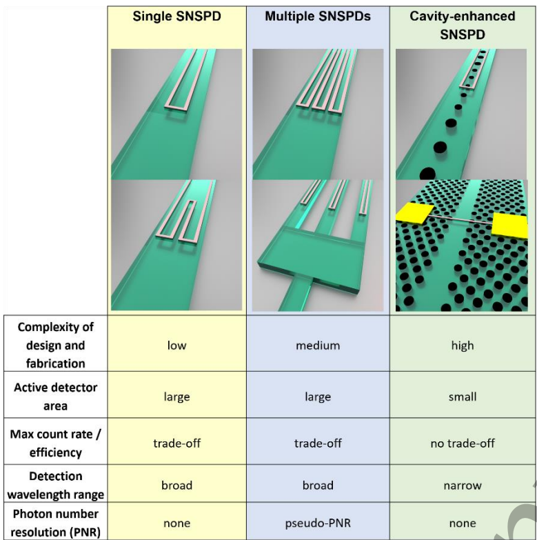
Figure 1 Device concepts for superconducting nanowire single photon detectors (SNSPDs) coupled to photonic integrated circuits (PIC). U- or W-shaped SNSPD coupled to a single waveguide (yellow). Multiple SNSPDs on a single waveguide or an array of waveguides (blue). SNSPDs coupled to one-dimensional and two-dimensional cavities (green).
