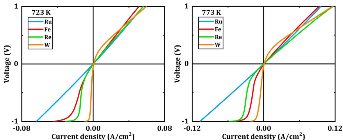
Figure 5. i -V polarization curves for the LST-BZCYYb cells with Pt on one side and either W, Re, Fe or Ru on the other at 723 K and 773 K. Scan rate was 0.01 V s -1 .
