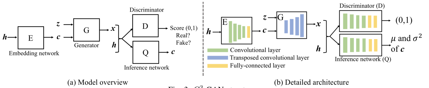
Fig. 3: C^3 -GAN structure.
