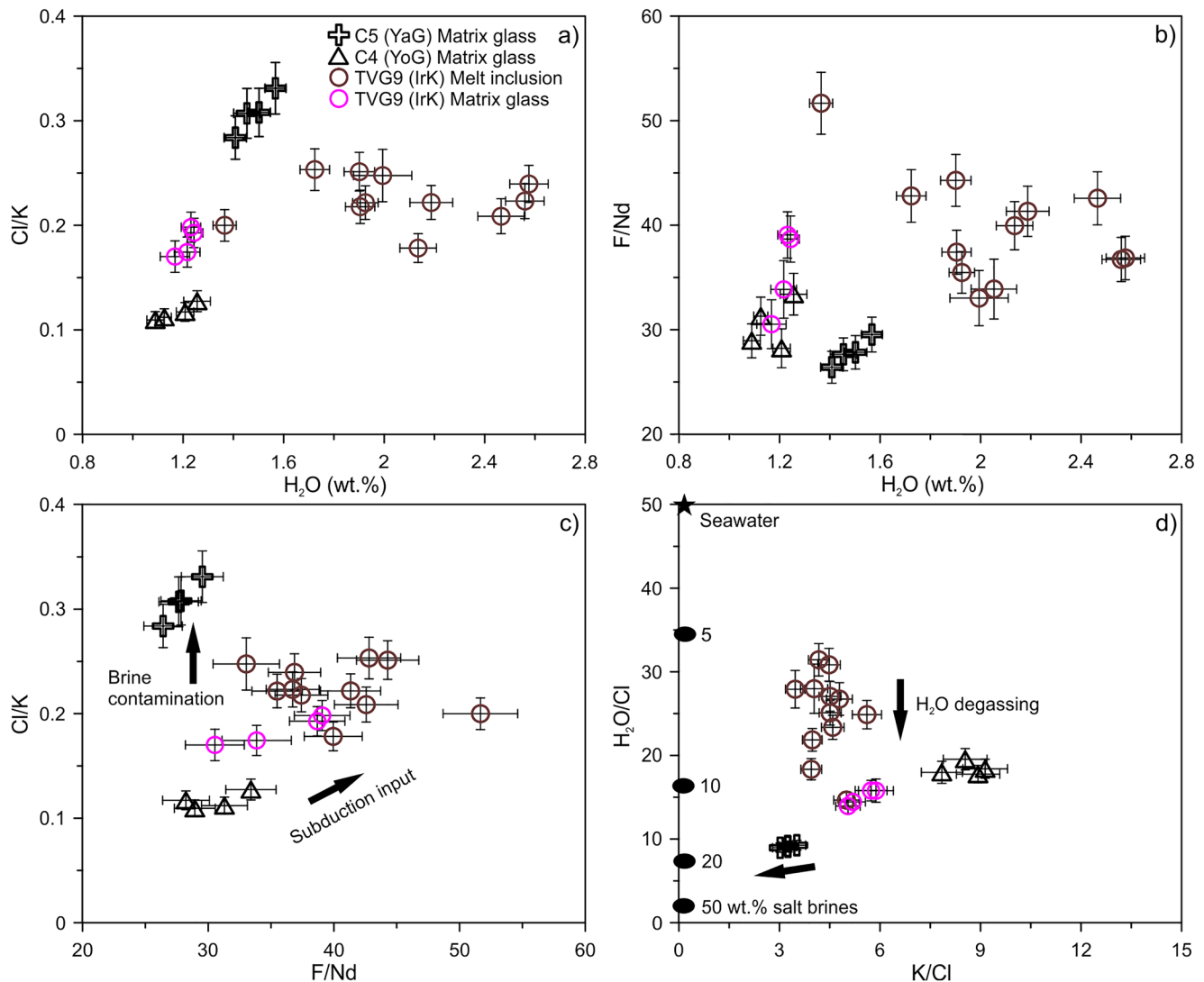
Figure 7. Plots of (a) Cl/K versus H 2 O, (b) F/Nd versus H 2 O, (c) Cl/K versus F/Nd, and (d) H 2 O/Cl versus K/Cl. The error bars indicate 2 \sigma uncertainties. The Yaeyama Graben (C5) lavas have much higher Cl/K ratio but lower F/Nd ratio, suggesting the brine contamination. The data of seawater and brines are from Kendrick et al. (2015). IrK, Irabu Knoll; YaG, Yaeyama Graben; YoG, Yonaguni Graben.
