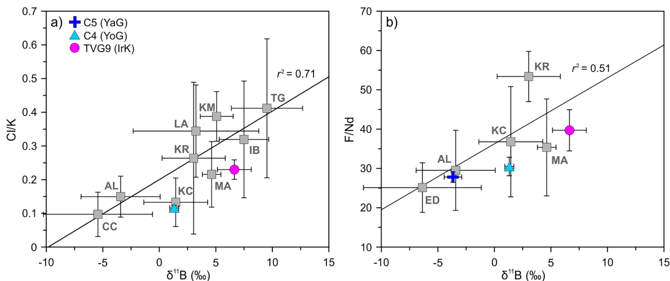
Figure 8. Plots of (a) Cl/K versus \delta^{11}\text{B} and (b) F/Nd versus \delta^{11}\text{B} for the lavas from southern Okinawa Trough lavas and 10 modern arcs (from GEOROC database: http://georoc.mpch-mainz.gwdg.de/georoc/ and Cooper et al., 2020; data with MgO > 4 wt.% were adopted). Each gray square represents the average values of each individual arc. The error bars indicate 1\sigma uncertainties. The arc average values are given Table S6 and the source data are given in Datasets. The linear positive correlations between \delta^{11}\text{B} and Cl/K, F/Nd for global arcs suggest serpentinite- ( \pm\text{AOC} -) derived fluids probably dominate the subduction input of halogens into the sub-arc mantle. AL, Aeolian; CC, Cascades; ED, Ecuador; IB, Izu-Bonin; IrK, Irabu Knoll; KC, Kamchatka; KM, Kermadec; KR, Kurile; LA, Lesser Antilles; MA, Mariana; TG, Tonga; YaG, Yaeyama Graben; YoG, Yonaguni Graben.
