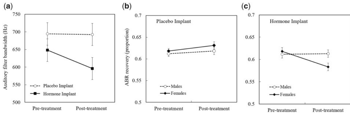
Fig. 2. (a) Frequency selectivity and (b, c) temporal resolution in house sparrows ( Passer domesticus ) treated with either a placebo or hormone implant ( N total = 36, N per group = 9). Frequency selectivity was measured using a notched-noise protocol to determine auditory filter bandwidth. Note that the bandwidths are averaged across center frequencies ( CF = 2, 3 , or 4 kHz) and that frequency selectivity is inversely related to filter bandwidth. Temporal resolution was measured with a paired click paradigm (inter-click intervals 0.7 – 25 ms). ABR (auditory brainstem response) recovery is the amplitude of the onset response to the second click divided by the amplitude of the onset response to a single click. (a) We did not find an effect of sex on frequency selectivity plasticity. Pre-treatment animals in the two treatment conditions did not differ. Animals with a placebo implant did not show plasticity in their frequency resolution (females: F_{1182} = 0.68 , P = 0.41 , males: F_{1182} = 0.68 , P = 0.41 ), but animals given a hormone implant showed enhanced frequency resolution after 3 weeks (females: F_{1182} = 5.7 , P = 0.018 , males: F_{1182} = 3.74 , P = 0.04 ). (b) Similarly, neither sex exhibited plasticity in temporal resolution when given a placebo implant (females: F_{1665} = 0.98 , P = 0.32 , males: F_{1665} = 0.3 , P = 0.59 ). (c) Females, but not males, showed diminished temporal resolution when given a hormone implant (females: F_{1665} = 21.7 , P < 0.001 , males: F_{1665} = 1.62 , P = 0.20 ). LSMEANS ( \pm SE) were generated in SAS 9.2.
