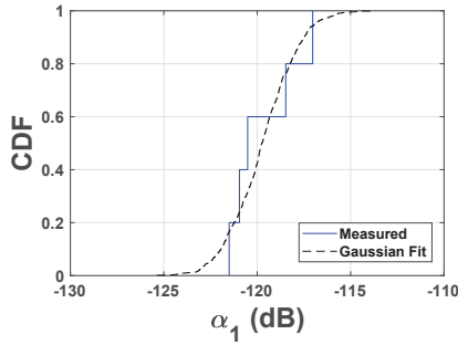
Fig. 6: CDF of DMC parameter \alpha_1 (dB) with Gaussian fit.
