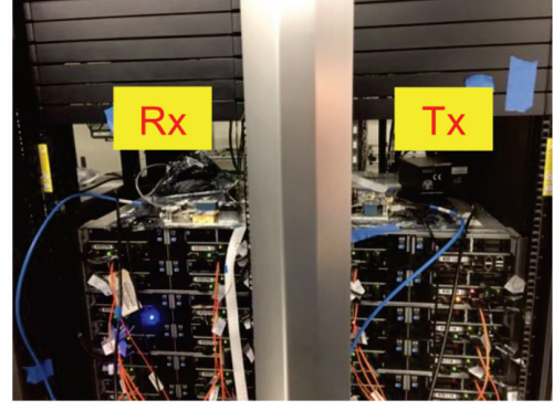
Fig. 2: Measurement setup in the LOS THz MIMO Channel.
