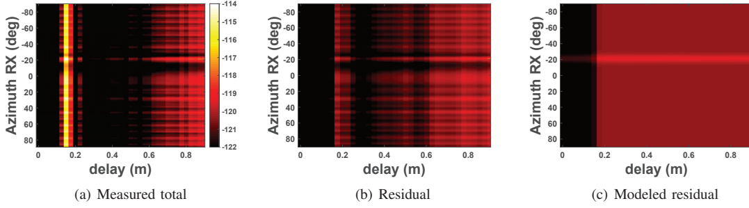
Fig. 5: PADP comparison at the RX from (a) measured channel, \mathbf{h} (b) residual channel, \mathbf{h} - (\mathbf{S}(\theta_{sp})) and (c) modeled DMC.
