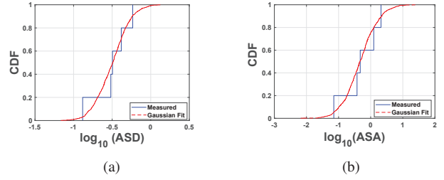
Fig. 3: CDF of (a) \log_{10}(\text{ASD}) and (b) \log_{10}(\text{ASA})
