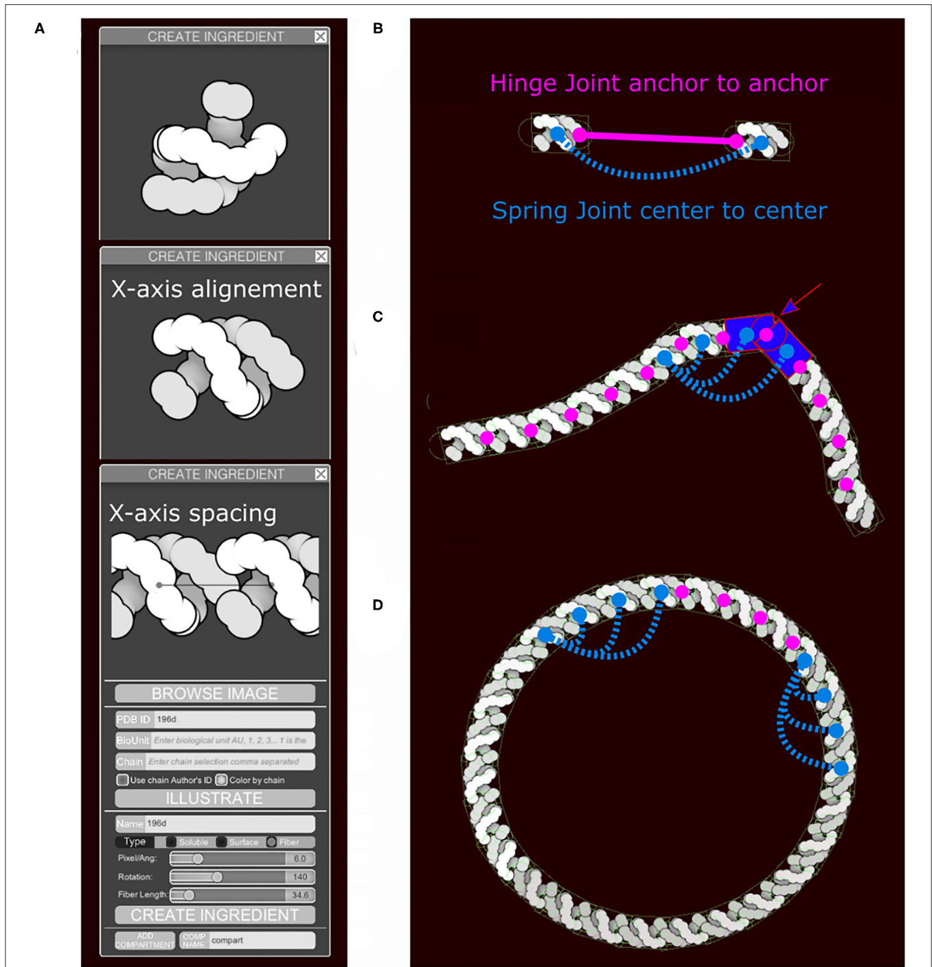
FIGURE 4 | Fiber generation and constraints. DNA structure from PDB ID 196D is used as an example. (A) Subunit is aligned by the user along the horizontal axis and a repetition/spacing distance is defined, using sliders in the user interface. (B) Two subunits are separated to illustrate the colliders and the joints in use. A rectangular main collider defines the steric properties of each subunit and is the anchor for the persistence length spring joint (blue). The two circular colliders at each end of the subunit serve as anchors for the hinge joint in magenta and do not see the colliders on the neighboring subunit. The hinge line length (magenta) will be constrained to be zero, the spring line length (blue) is always proportional to the spacing times N , the neighbors index defining the number of segments. (C) The DNA fiber with proper spacing, illustrating the second role of the circle collider (arrow) that fills the gap for acute angle between subunit. (D) Circular DNA showing the role of the spring joints in maintaining a persistence length.
