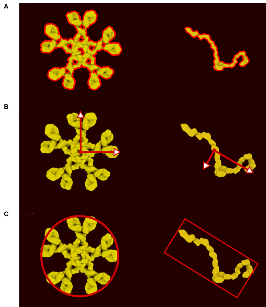
FIGURE 3 | Definition of colliders. (A) 2D polygon collider defined from the image contour. (B) Eigenvector and eigenvalue calculated from the polygon vertices. (C) Main proxy collider chosen from the eigenvector.
