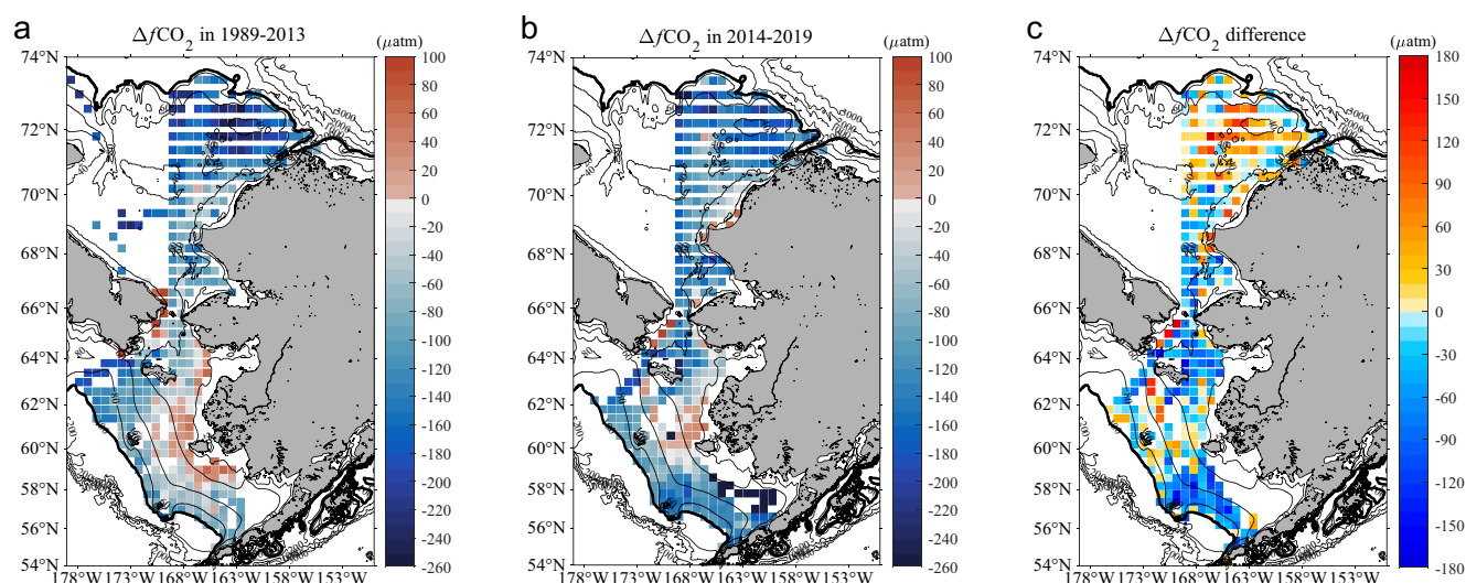
Figure 7. Gridded means surface \Delta f\text{CO}_2 at 0.8^\circ (longitude) \times 0.4^\circ (latitude) in the periods of (a) 1989–2013, (b) 2014–2019, and (c) the difference between these two periods.
