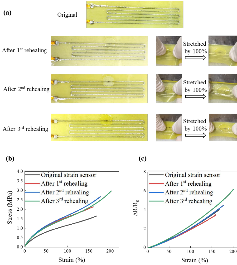
Fig. S6. (a) Optical images of the original strain sensor (top) and after cutting and rehealing for once (second row), twice (third row) and three times (bottom). The rehealed strain sensor can be stretched by 100%. (b) Stress-strain curves of the original and rehealed strain sensors. (c) Relative resistance change \Delta R/R_0 of the original and rehealed strain sensors versus applied uniaxial strain.
