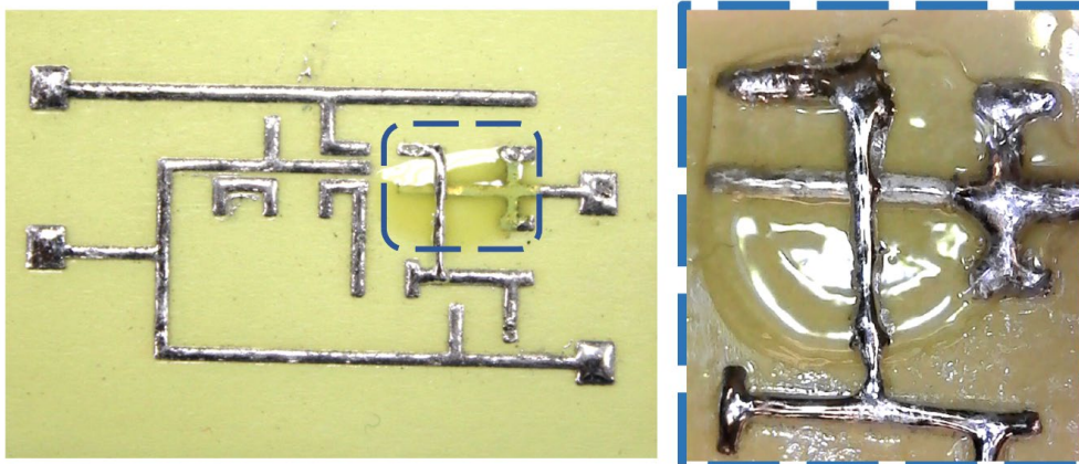
Figure S8: The amplifying circuit without chip components (left). Enlarged microscope image shows details of intersections of LM wires (right).
