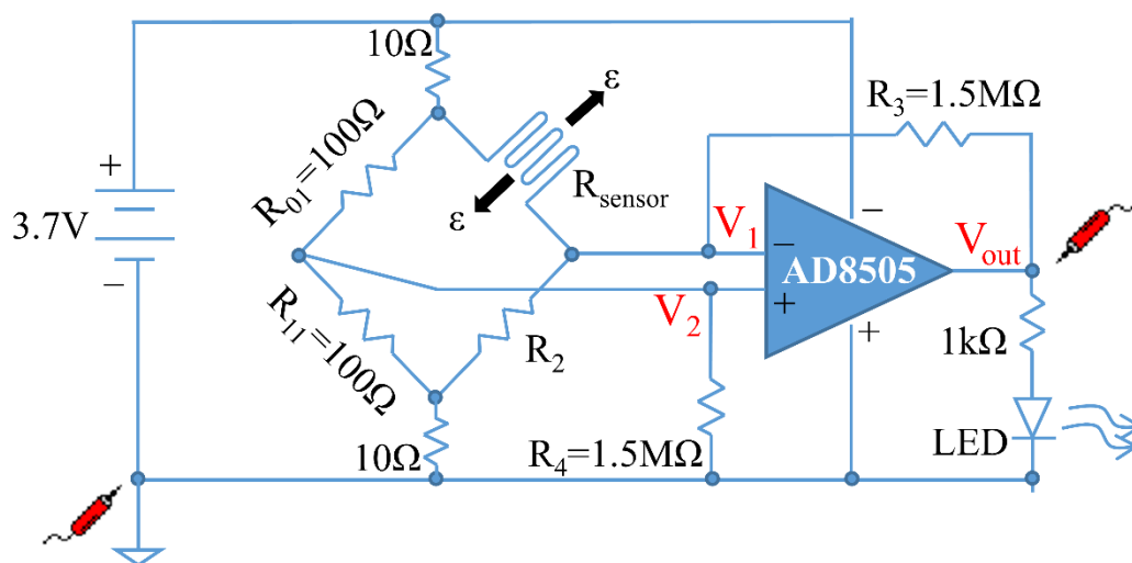
Figure S9: Wheatstone bridge differential amplifier circuit.
