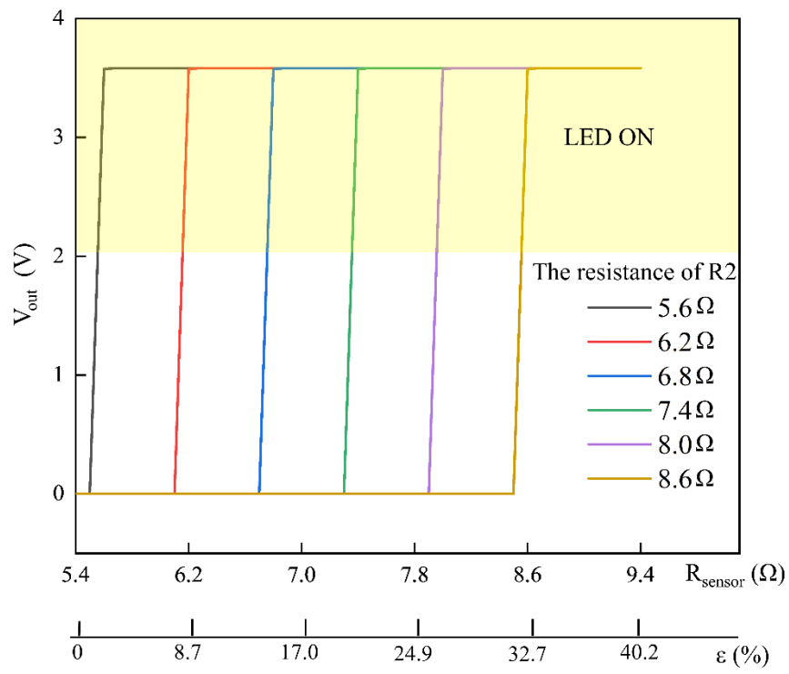
Figure S10: Simulated V_{out} versus R_{sensor} and the strain \epsilon applied to the strain sensor.
