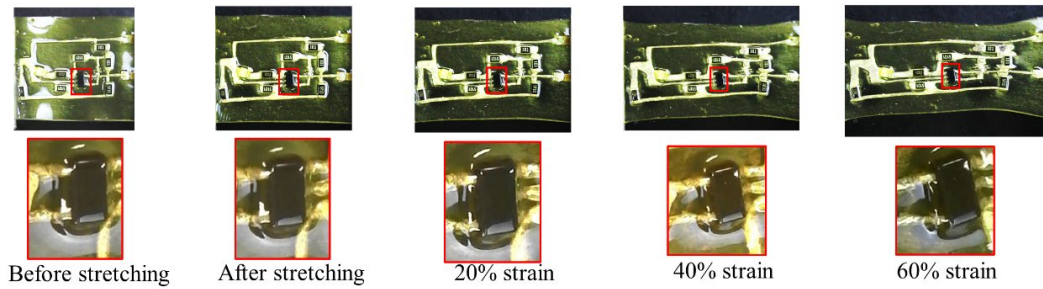
Figure S3: Optical images of the amplifying circuit under uniaxial stretching. The second image shows the device after release of the strain, to illustrate reversibility in the responses. Microscope images of op-amplifier at the bottom show no signs of debonding or failure in LM interconnects.
