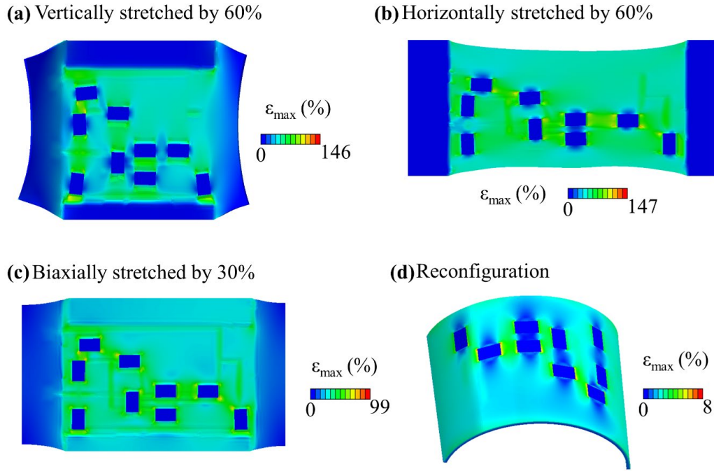
Figure S2: Max principal strain contours in polyimine when the amplifying circuit is subjected to 60% uniaxial strain along vertical (a) and horizontal (b) directions, 30% biaxial strain (c), and reconfiguration (d).
