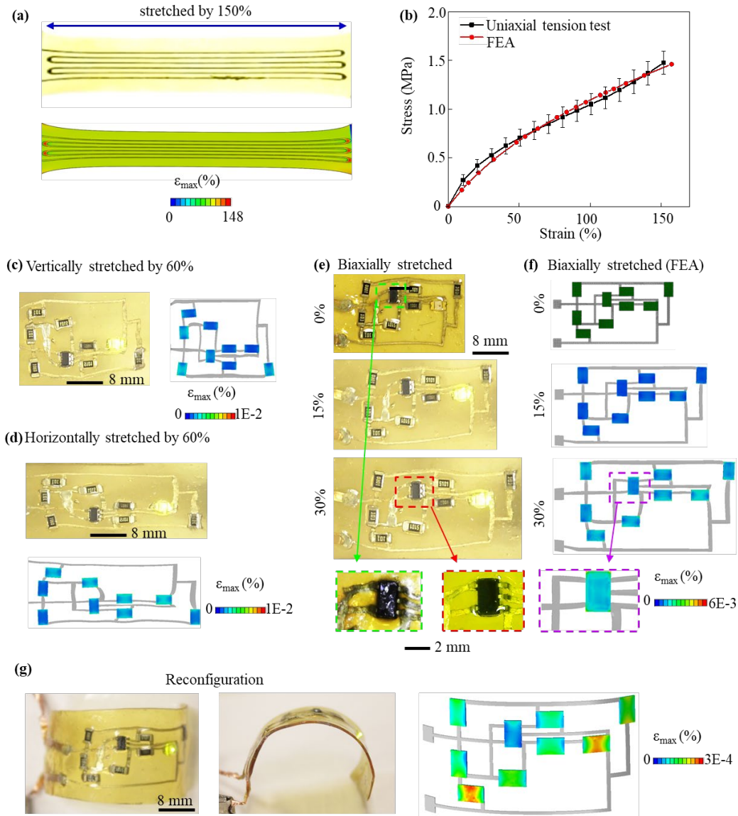
Figure 2: Mechanical properties of the strain sensor and amplifying circuit. (a) Optical image (top) and FEA strain contour (bottom) of the strain sensor stretched by 150%. (b) Uniaxial stress-strain curves of the strain sensor obtained from experiment and FEA. (c) Optical image (left) and FEA strain contour (right) of the amplifying circuit vertically stretched by 60%. (d) Optical image (top) and FEA strain contour (bottom) of the amplifying circuit horizontally stretched by 60%. (e) Optical images of the amplifying circuit at 0% strain (top), biaxially stretched by 15% (middle), and biaxially stretched by 30% (bottom). The two insets show microscope images of a chip component at undeformed and biaxially stretched by 30% states. (f) FEA simulation model of the amplifying circuit (top), and strain contours of the amplifying circuit biaxially stretched by 15% (middle) and 30% (bottom). (g) The amplifying circuit can be reconfigured to a cylindrical shape (left: top view, middle: side view). FEA simulation gives the strain contour in chip components in the cylindrical shape (right).
