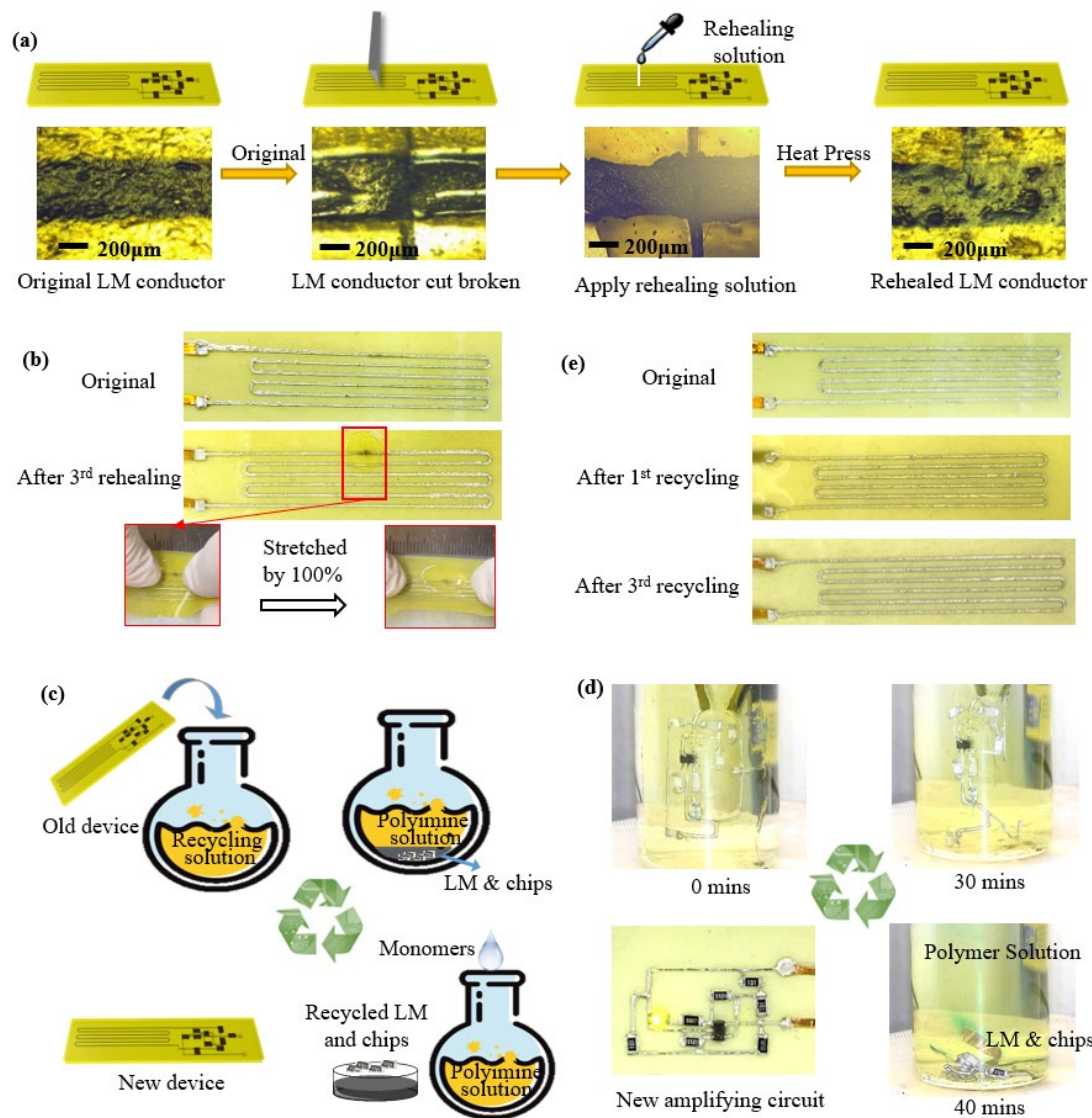
Figure 3: Rehealing and recycling of the device. (a) Schematic illustration (top) and experimental microscope images (bottom) of the rehealing process. (b) Optical images of the original strain sensor (top) and after cutting and rehealing for three times (middle). The rehealed strain sensor can be stretched by 100% (bottom). (c) Schematic illustration of the recycling process. (d) Optical images of the recycling of an amplifying circuit. (e) Optical images of the original strain sensor (top) and after recycling for once (middle) and three times (bottom).
