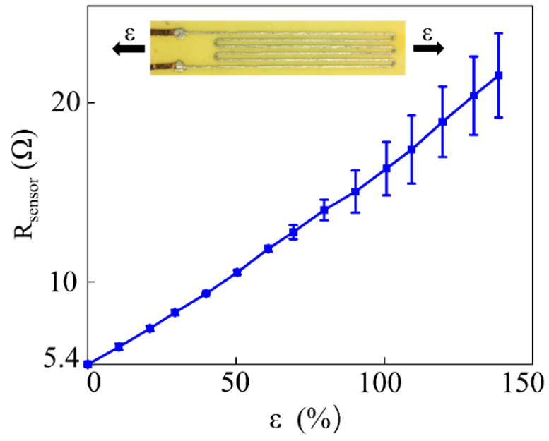
Figure S5: Resistance change of the strain sensors versus applied uniaxial strain.
