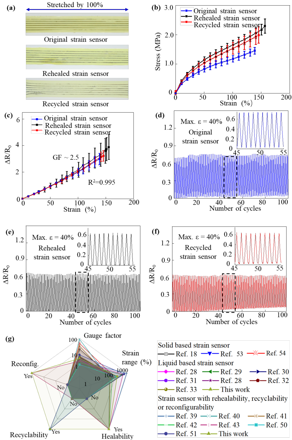
Figure 4: Characterization of the rehealed and recycled strain sensor. (a) Optical images of the original (top), rehealed (middle) and recycled (bottom) strain sensor stretched by 100%. (b) Stress-strain curves of the original, rehealed and recycled strain sensors. (c) Relative resistance change \Delta R/R_0 of the original, rehealed and recycled strain sensors versus applied uniaxial strain. Relative resistance change \Delta R/R_0 of the original (d), rehealed (e) and recycled (f) strain sensor under cyclic loading. The maximum strain is 40%. The insets exhibit magnified views of 10 cycles between cycle numbers 45 and 55. (g) Comparison of this work with previously reported stretchable strain sensors.
