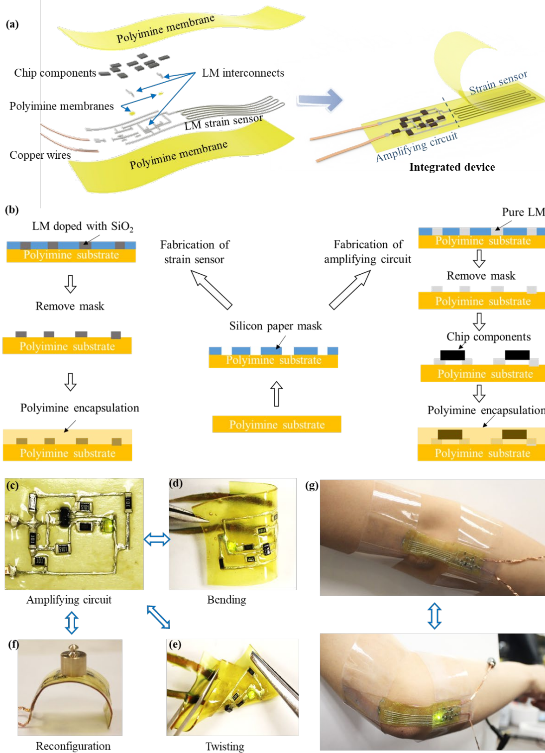
Figure 1: Design, construction and fabrication of the stretchable strain sensing system. (a) Exploded view of the strain sensing system. (b) Schematic illustration of the fabrication processes of the amplifying circuit and strain sensor. Optical images of the amplifying circuit in its undeformed (c), bent (d), and twisted (e) states. (f) Reconfiguration of the amplifying circuit. (g) The strain sensing system is attached on an elbow for monitoring its flexion states. When the elbow is straight, the LED is off (top). When the elbow flexes beyond a threshold, the LED turns on (bottom).
