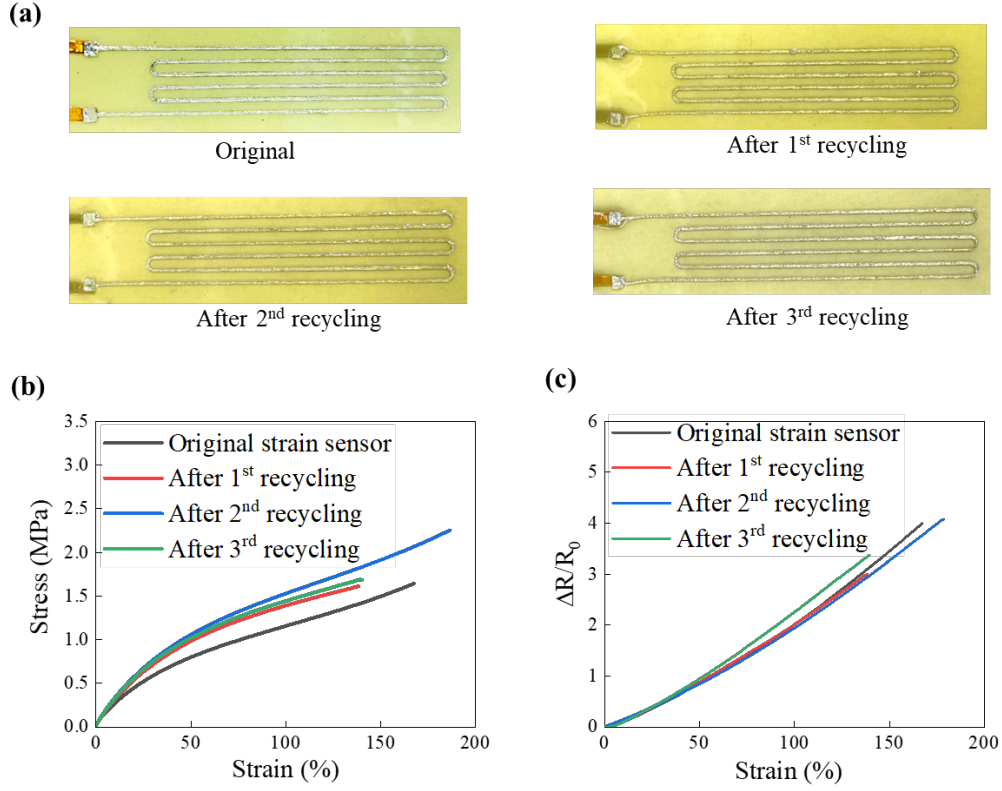
Fig. S7. (a) Optical images of the original strain sensor (top left) and after recycling for once (top right), twice (bottom left) and three times (bottom right). (b) Stress-strain curves of the original and recycled strain sensors. (c) Relative resistance change \Delta R/R_0 of the original and recycled strain sensors versus applied uniaxial strain.
