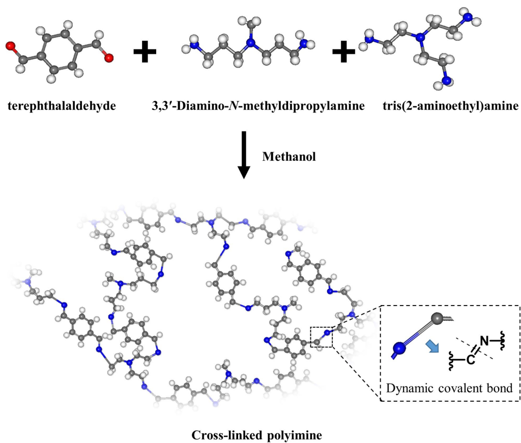
Figure S1: Preparation of polyimine network through imine condensation reaction.
