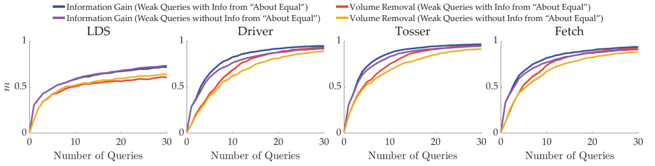
Figure 16. The results (mean \pm s.e.) of the simulations with weak preference queries where we use the information from “About Equal” responses (blue and red lines) and where we don’t use (purple and orange lines).
