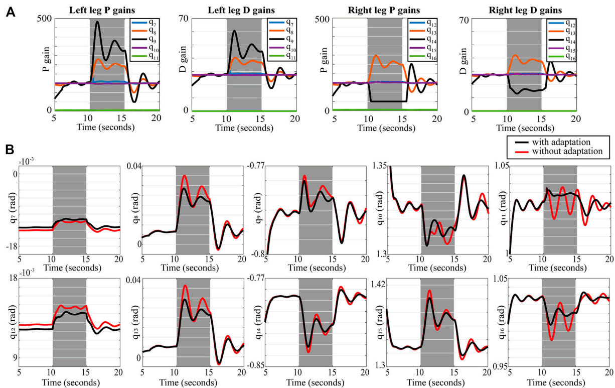
FIGURE 4 | Simulation results of pushing the pelvis: (A) The adapted gains of the WBLC in the joint level. (B) The configuration of the robot controlled by WBLC.
