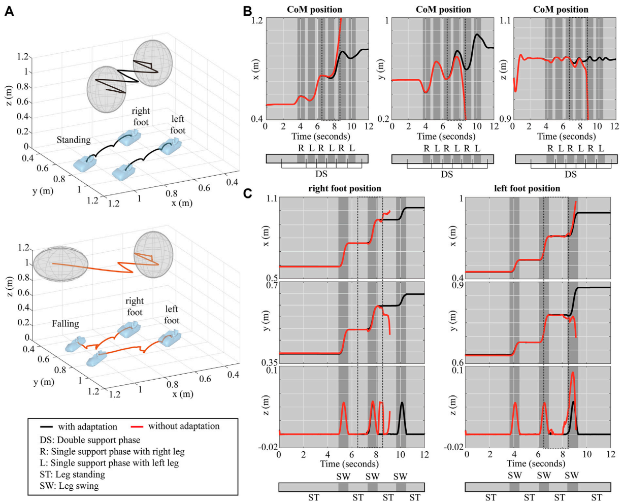
FIGURE 11 | Simulation results of walking with an external force: (A) positions of CoM and feet in Cartesian coordinate, (B) the robot's CoM position, (C) the robot's feet positions.
