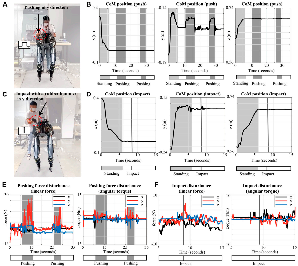
FIGURE 9 | Experiment results with the same scenarios with the simulations in 4.1.1 and 4.1.3: pushing (A,B) and impacting (C,D) the pelvis of Draco2 in double support phase. The estimated external disturbance \mathbf{F}_t is computed when pushing (E) and impacting (F) the robot.
