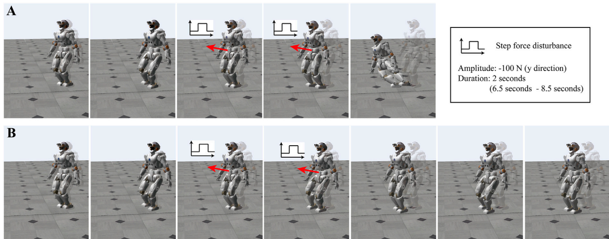
FIGURE 10 | Snapshots of simulations for walking while an external force exists: (A) walking without the proposed gain adaptation, (B) walking with the online gain adaptation.
