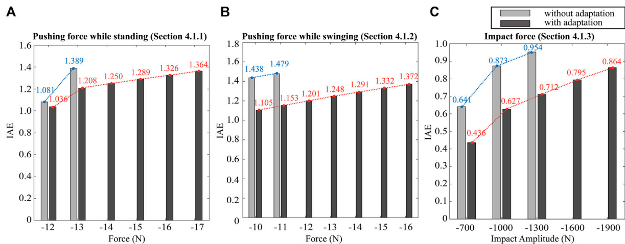
FIGURE 7 | IAE values corresponding to simulation results with different levels of external disturbances: The simulation scenarios are those described in Sections 4.1.1 (A), 4.1.2 (B), and 4.1.3 (C) . To calculate the IAE values of the impact simulation (C) , we use the same time interval [10, 15] to cases (A,B) .
