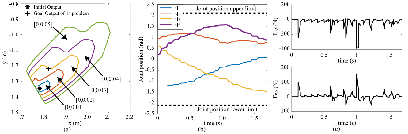
Fig. 2. (a) Non-convex hull of the reachable output set within the time interval: N\text{conv}(\overline{\mathcal{R}}_{[0,T]}^y(x_0)) , (b) joint position trajectory, (c) contact force
