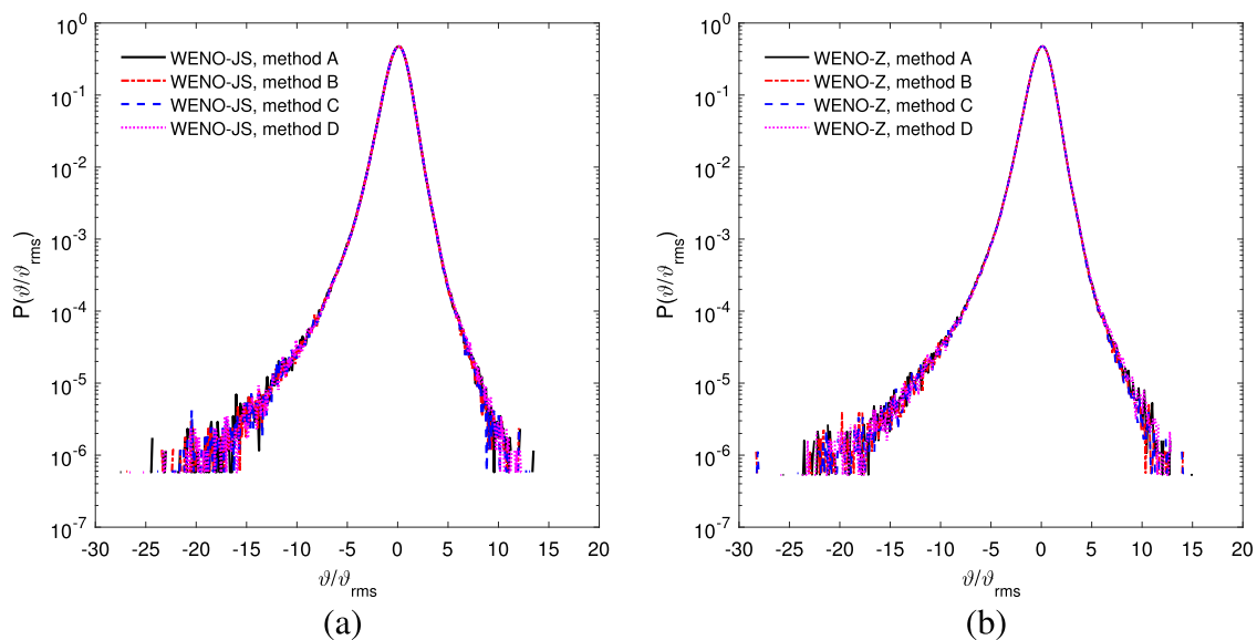
FIG. 16. Comparison of the PDF of normalized velocity divergence by using methods A–D at t/T_e = 1.56 . (a) WENO-JS combined with methods A–D and (b) WENO-Z combined with methods A–D.
