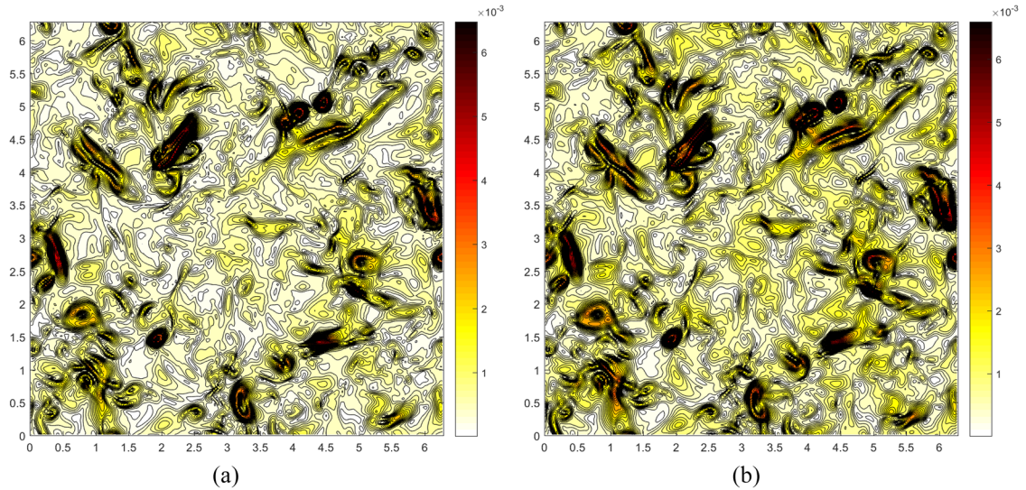
FIG. 14. Slices of contours of the (a) density-based local Knudsen number Kn_p and (b) pressure-based local Knudsen number Kn_p at t/T_e = 1.56 .
