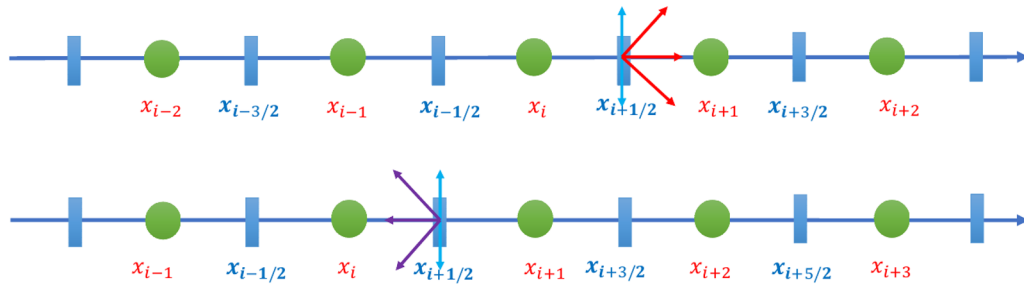
FIG. 25. The fifth-order WENO scheme for the reconstruction of particle distribution functions at the cell interface.
