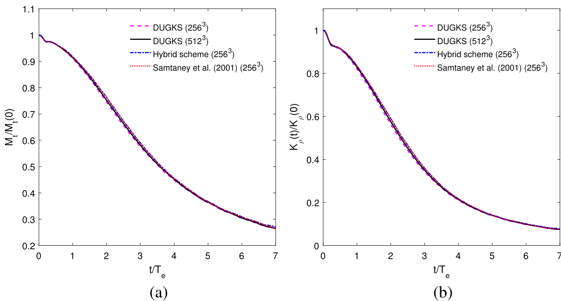
FIG. 10. (a) Time evolution of the turbulent Mach number Ma_t/Ma_0 . (b) Time evolution of normalized turbulent kinetic energy K_p(t)/K_p(0) .
