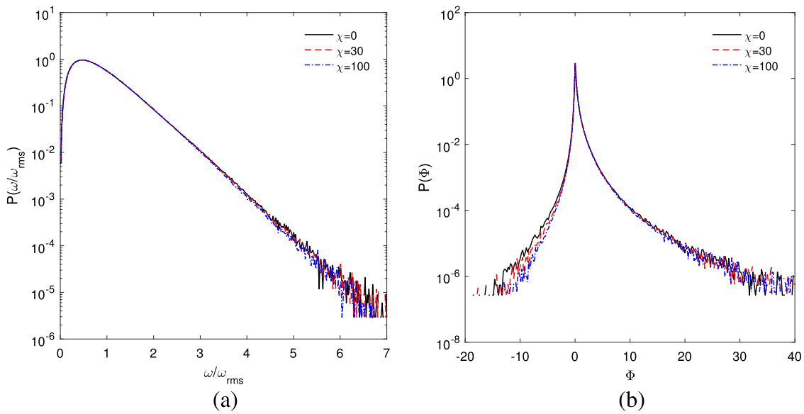
FIG. 22. (a) PDF of normalized vorticity magnitude \omega/\omega_{rms} . (b) PDF of normalized vortex stretching term \Phi = (\omega \cdot S \cdot \omega) / (\langle \omega^2 \rangle \langle S : S \rangle^{1/2}) . Time t/T_e = 1.56 .
