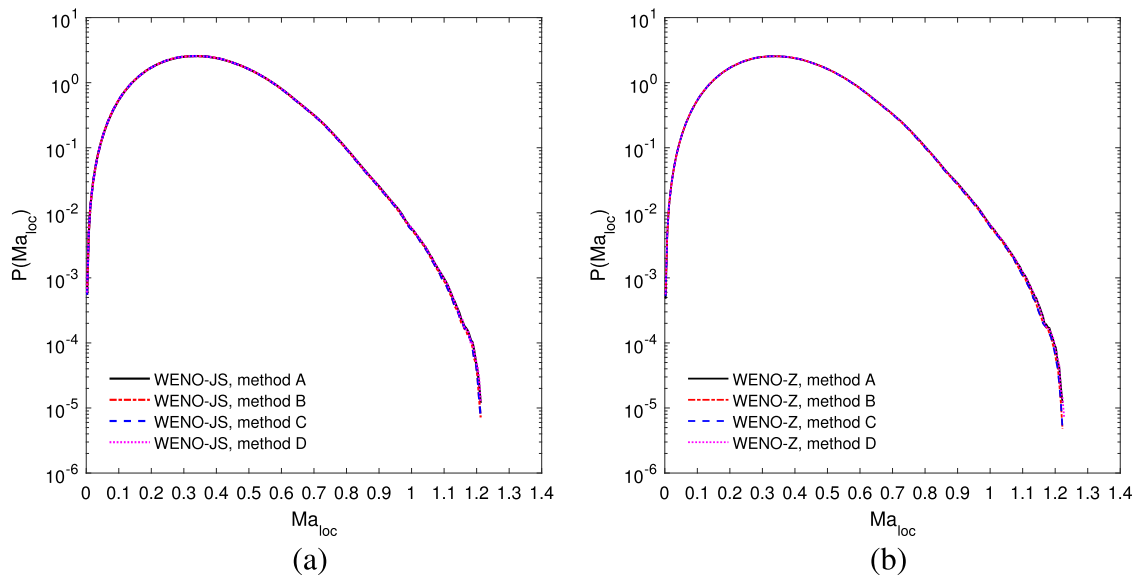
FIG. 15. Comparison of the PDF of the local Mach number by methods A–D at t/T_e = 1.56 . (a) WENO-JS combined with methods A–D and (b) WENO-Z combined with methods A–D.
