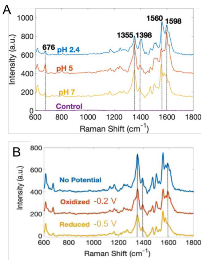
Figure 5. Surface-enhanced Raman spectra of PYO as a function of (A) pH, and (B) electrochemical potential. Adapted with permission from ref 121 . Copyright 2019 American Chemical Society.
