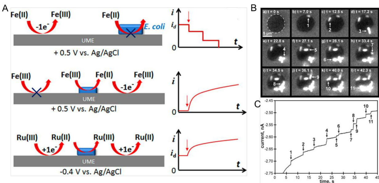
Figure 6. (A) Different ways of detecting bacteria-electrode collisions along with their current-time responses. Top panel: bacterial cell blocking the UME electroactive area; Middle panel: bacterial cell catalyzing reduction; Bottom panel: regeneration of redox species by bacterial cell. (B) Time-lapse fluorescence images showing E. coli attaching to the UME surface. (C) Current-time trace corresponding to panel B. Panel A is adapted with permission from ref 130 . Copyright 2018 American Chemical Society. Panels B and C are adapted with permission from ref 129 . Copyright 2018 Elsevier Ltd.
