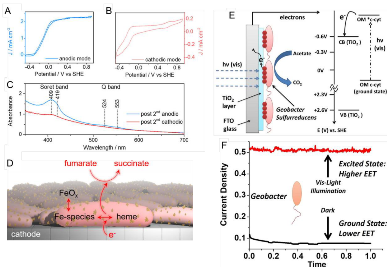
Figure 2. Cyclic voltammograms of a G. sulfurreducens biofilm on an indium-tin-oxide (ITO) electrode in (A) anodic (acetate to CO 2 ) and (B) cathodic (fumarate to succinate) modes. (C) UV-visible spectra of biofilms after anodic and cathodic scans. (D) Schematic illustrating plausible EET mechanism in cathodic mode. (E) Schematic and energy diagram showing EET from G. sulfurreducens directly to TiO 2 under visible illumination. OM = outer membrane. (F) Current density obtained from G. sulfurreducens under dark and illuminated conditions. Panels A-D are adapted with permission from ref 66 . Copyright 2020 American Chemical Society. Panel E and F are adapted with permission from ref 70 . Copyright 2020 Elsevier B.V.
