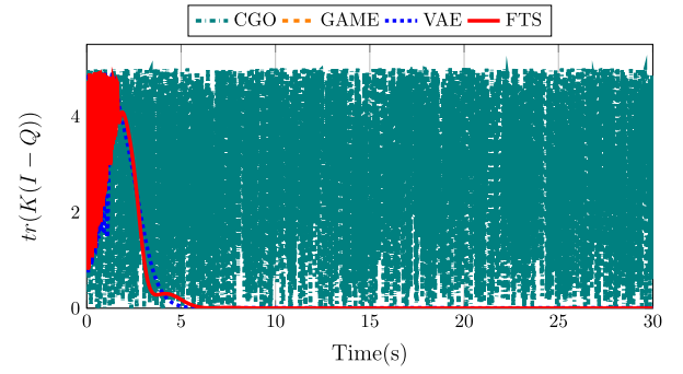
Fig. 3. Attitude estimation error for low noise levels, with estimator gains unchanged.
