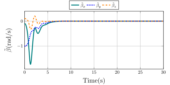
(c) Bias estimation error \hat{\beta} with time
