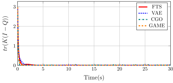
Fig. 2. Attitude estimation error for noise levels similar to that in Zamani (2013).
