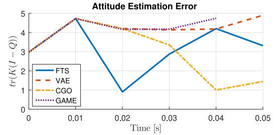
Fig. 4. Zoomed-in view of the initial transient response of the attitude estimation error as plotted in Fig. 3.
