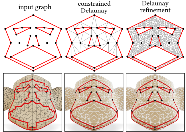
Fig. 25. Top. Planar constrained Delaunay triangulations are used to produce high-quality triangulations which conform to a collection of specified lines. Bottom. Constrained intrinsic triangulations play a similar role on surfaces, preserving a set of intrinsic edges in the triangulation.
