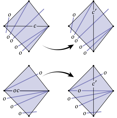
Fig. 19. Flipping an edge in the explicit crossing representation [Fisher et al. 2007].
