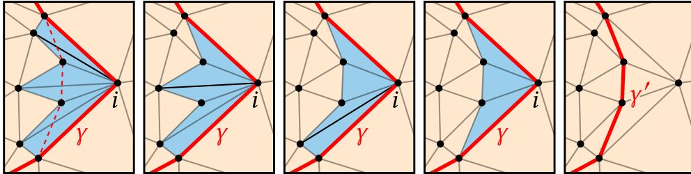
Fig. 33. FLIPOUT shortens the curve \gamma by repeatedly flipping edges to introduce a shorter path.
