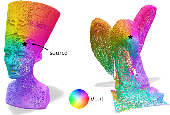
Fig. 43. Angular parameterizations of point clouds, computed with the tufted intrinsic Delaunay point cloud Laplacian via the vector heat method [Sharp et al. 2019c].
