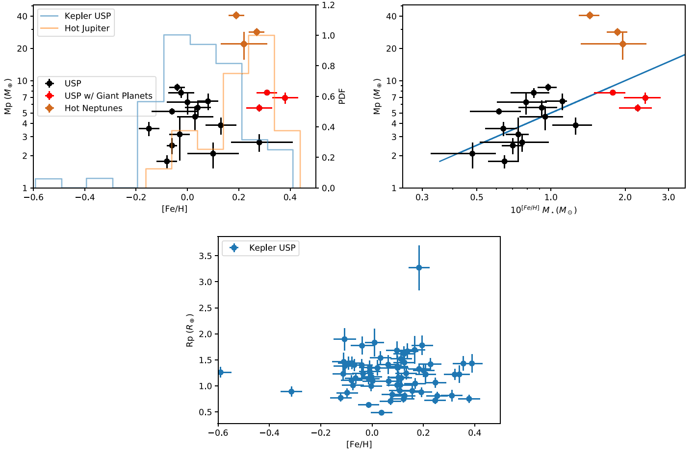
Figure 12. Top left: the metallicity vs. planet mass of USPs (black) and ultrahot Neptunes (brown) with mass and radius measurements. The histograms are the metallicity distribution of all Kepler USPs (blue) and hot Jupiters (orange). Top-right: a proxy for disk solid density 10^{[\text{Fe}/\text{H}]} M_\star vs. the planet mass of USPs (black) and ultrahot Neptunes (brown). The implicit assumption is that protoplanetary disk density scales linearly host-star mass and solid surface density scales with host-star metallicity. A statistically strong ( p = 0.04 ) correlation is observed. The blue line shows a linear scaling between 10^{[\text{Fe}/\text{H}]} M_\star and M_p . Bottom: the radii and host metallicity of the uniformly studied USP sample from Kepler (Sanchis-Ojeda et al. 2014). Only 1 out of 67 is in the Neptune-radius regime (KOI-3913), suggesting that ultrahot Neptunes are likely much rarer than USPs. Also note KOI-3913’s relatively high metallicity similar to the confirmed ultrahot Neptunes.
