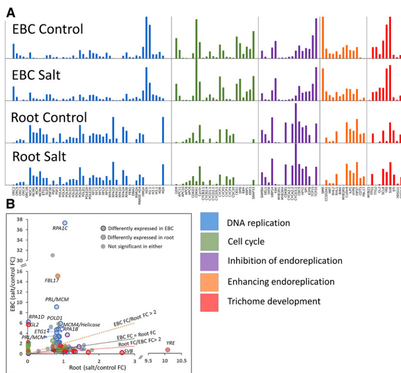
Figure 8. Differential responses of selected genes to salt stress in root and EBC transcriptomes. A, Normalized expression values within a category scaled from 0 to 1 on the y axis. B, Fold change (FC) between salt and control treatments.
