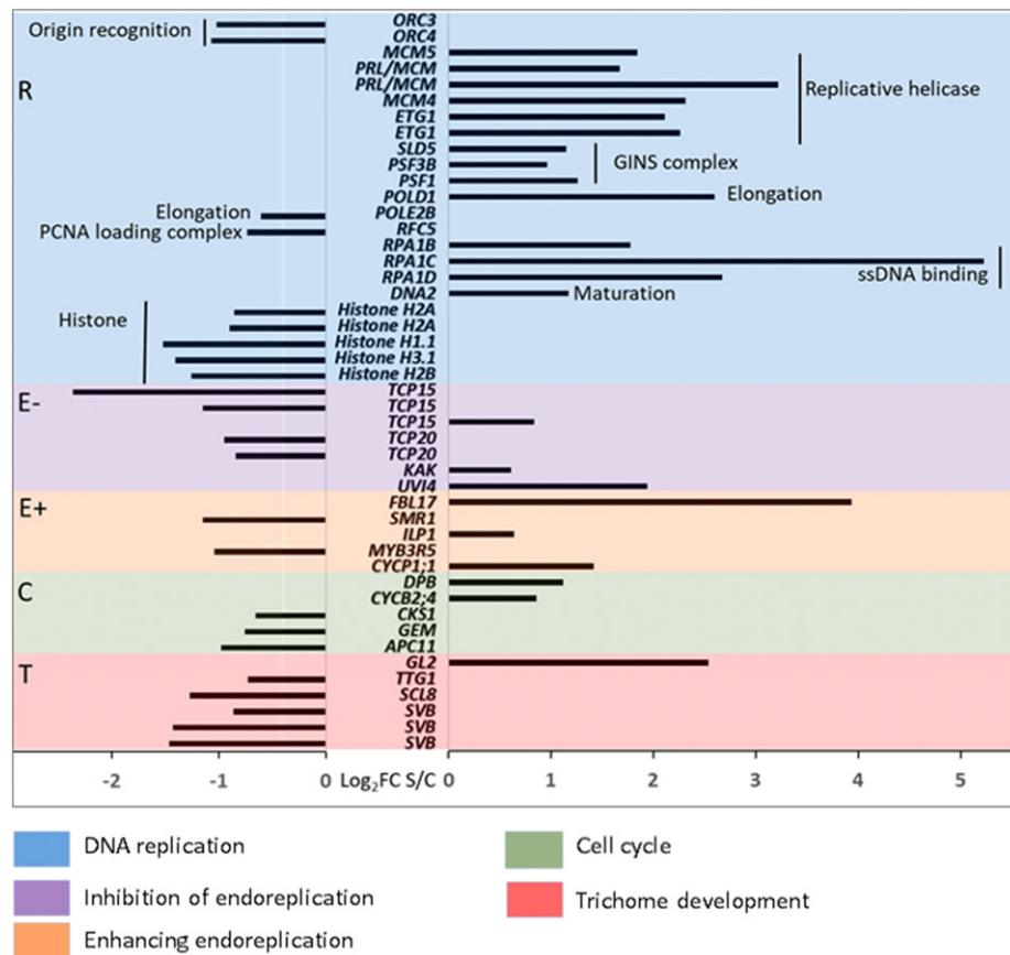
Figure 7. Fold change ( \log_2 ) of significantly differentially expressed genes associated with endoreplication in the M. crystallinum bladder cell transcriptome in response to 200 mM NaCl. Significantly different expression was evaluated at an adjusted P < 0.05 and false discovery rate = 0.01.
