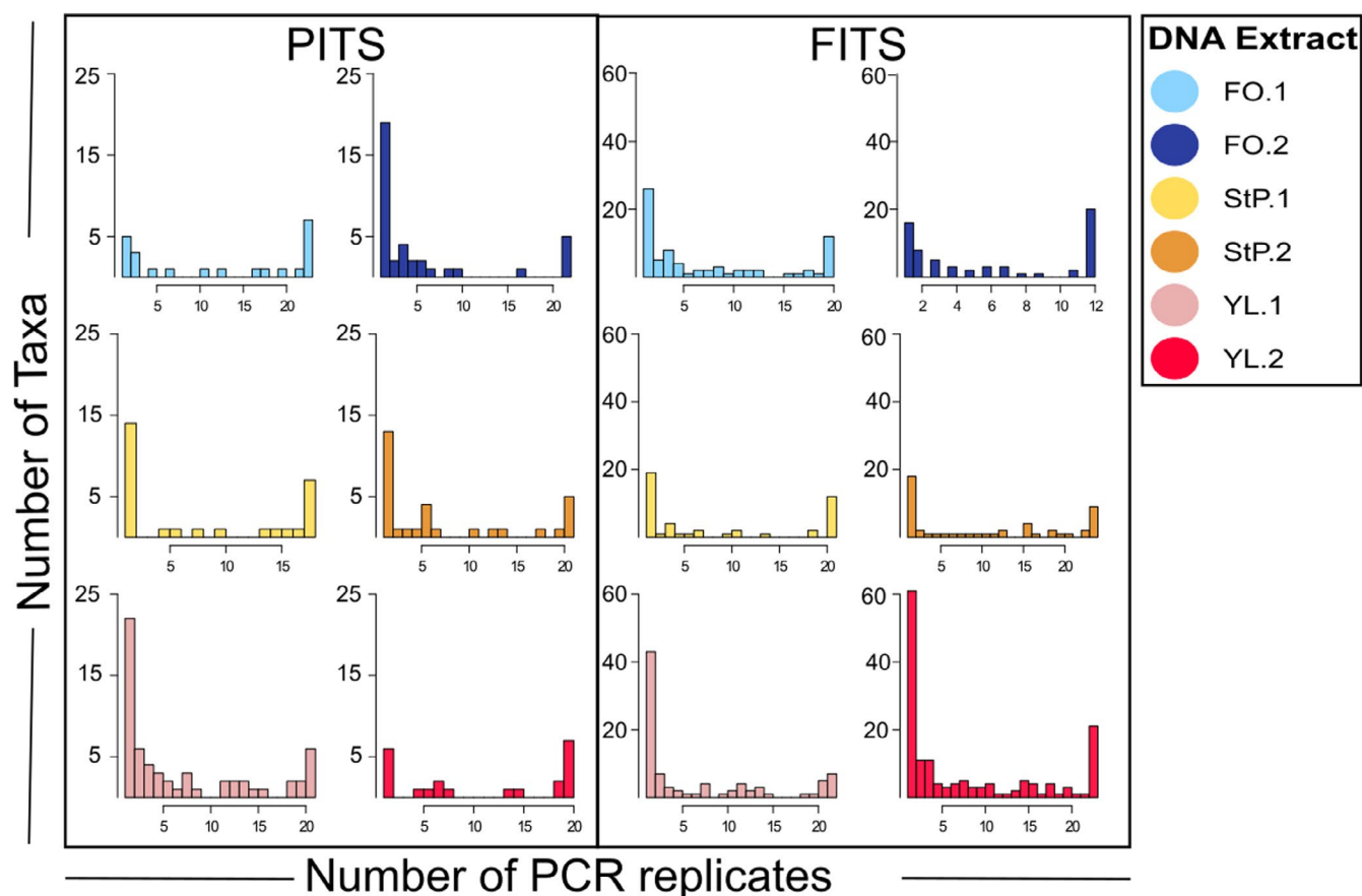
FIGURE 4 Histograms describing the frequency of individual taxa detected across PCR replicates, each sampled to a read depth of 5000 reads and using a minimum read threshold of five, out of the total 24 replicates. The right-most bar in each plot is a count of taxa present in all replicates, while the left-most bar is a count of taxa present in only one replicate
