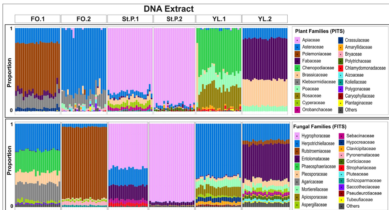
FIGURE 6 Relative abundance of plant and fungal families detected with 5000 reads and a five read minimum threshold. Each bar represents one PCR replicate. Only the 20 most abundant families are included here
