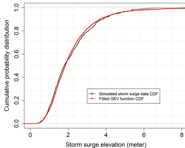
Fig. 2. The fitted cumulative distribution of storm surge height in Bay County.
