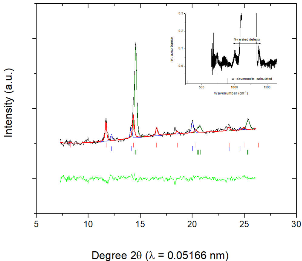
Fig. 1. X-ray diffraction pattern and Rietveld refinement of davemaoite. Red: davemaoite (dvm) olive: (Fe,C), blue: wüstite (wüs), green: residual of fit. Tick marks indicate allowed reflections (same colour-coding). R_{wp} was 0.046 and R_F for dvm was 0.10. Phase proportions were 35(5), 45(5), and 15(5)% for dvm, (FeC), and wüs, respectively. In dvm the intensity of reflections 100 and 201 indicates sublattice disorder of with A-cations shifted from site 1b to the 1/8-occupied site 8g. This is consistent with accommodation of K and Na along with Al and Fe. The paragenesis was found in two inclusions. Volumes of analyzed davemaoite inclusions ranged from 45.1 to 46.3 Å 3 (equal to 0 – 6 GPa (7) in pure CaSiO 3 ), but the actual composition of
