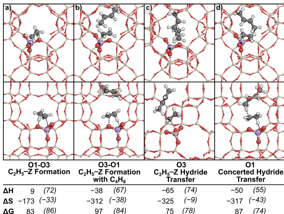
Fig. 3. Lowest energy transition state of a) \text{C}_2\text{H}_5\text{-Z} formation, b) \text{C}_2\text{H}_5\text{-Z} formation with spectating \text{C}_4\text{H}_8 , c) \text{C}_2\text{H}_5\text{-Z} hydride transfer, and d) concerted hydride transfer in CHA. Effective enthalpy ( \Delta H , \text{kJ mol}^{-1} ), entropy ( \Delta S , \text{J mol}^{-1} \text{ K}^{-1} ), and free energy ( \Delta G , \text{kJ mol}^{-1} ) barriers are reported at 433 K and relative to a bare acid site (proton) and stoichiometric amounts of gas-phase \text{C}_2\text{H}_4 and \text{C}_4\text{H}_8 . Intrinsic enthalpy, entropy, and free energy barriers are also given as ( \Delta E_{\text{act}} ) in italics. Dashed lines represent breaking and forming bonds.
