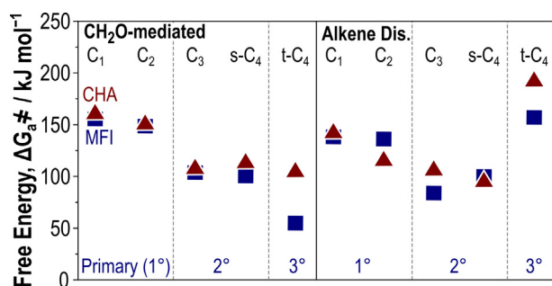
Fig. 10. Free energy ( \Delta G_a^\ddagger ) barriers ( \text{kJ mol}^{-1} ) for \text{C}_1 (methyl), \text{C}_2 (ethyl), \text{C}_3 (propyl), s\text{-C}_4 (sec-butyl), and t\text{-C}_4 (tert-butyl) reaction via \text{CH}_2\text{O} -mediated (left) and alkene-mediated routes (right) in MFI (blue, squares) and CHA (red, triangles). Reactions mediated by primary ( 1^\circ ), secondary ( 2^\circ ), and tertiary ( 3^\circ ) carbocations are grouped. Transition state structures associated with these states are shown in Section S8. (For interpretation of the references to colour in this figure legend, the reader is referred to the web version of this article.)
