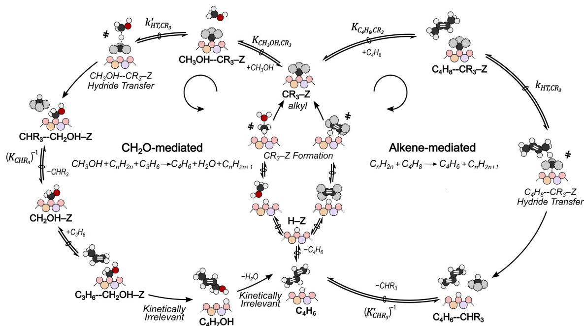
Scheme 3. Abbreviated mechanism of alkene-mediated and \text{CH}_2\text{O} -mediated diene formation routes demonstrating that surface-bound alkyls can participate in two competing hydride transfer mechanism. Steps shown with gray substituents, R, represent H, \text{CH}_3 , or \text{CH}_2\text{CH}_3 . Rate constants ( k and K ) used in Equations (13) and (15) are defined here. Surface-bound alkyls can be formed from either \text{CH}_3\text{OH} (to form \text{CH}_3\text{-Z} ) or an alkene, such as \text{C}_2\text{H}_4 (which forms \text{C}_2\text{H}_5\text{-Z} ). Alkyl species are represented as \text{CR}_3\text{-Z} and in the case of the alkene formation route, at least one R group will be -\text{CH}_3 or -\text{C}_2\text{H}_5 . The hydride transfer transition state for each pathway ( \text{CH}_3\text{OH-CR}_3\text{-Z} and \text{C}_4\text{H}_8\text{-CR}_3\text{-Z} ) is the transition state used to calculate \Delta G_a^\ddagger (Eq. (12)) relative to the \text{CR}_3\text{-Z} state and corresponding gas-phase species.
