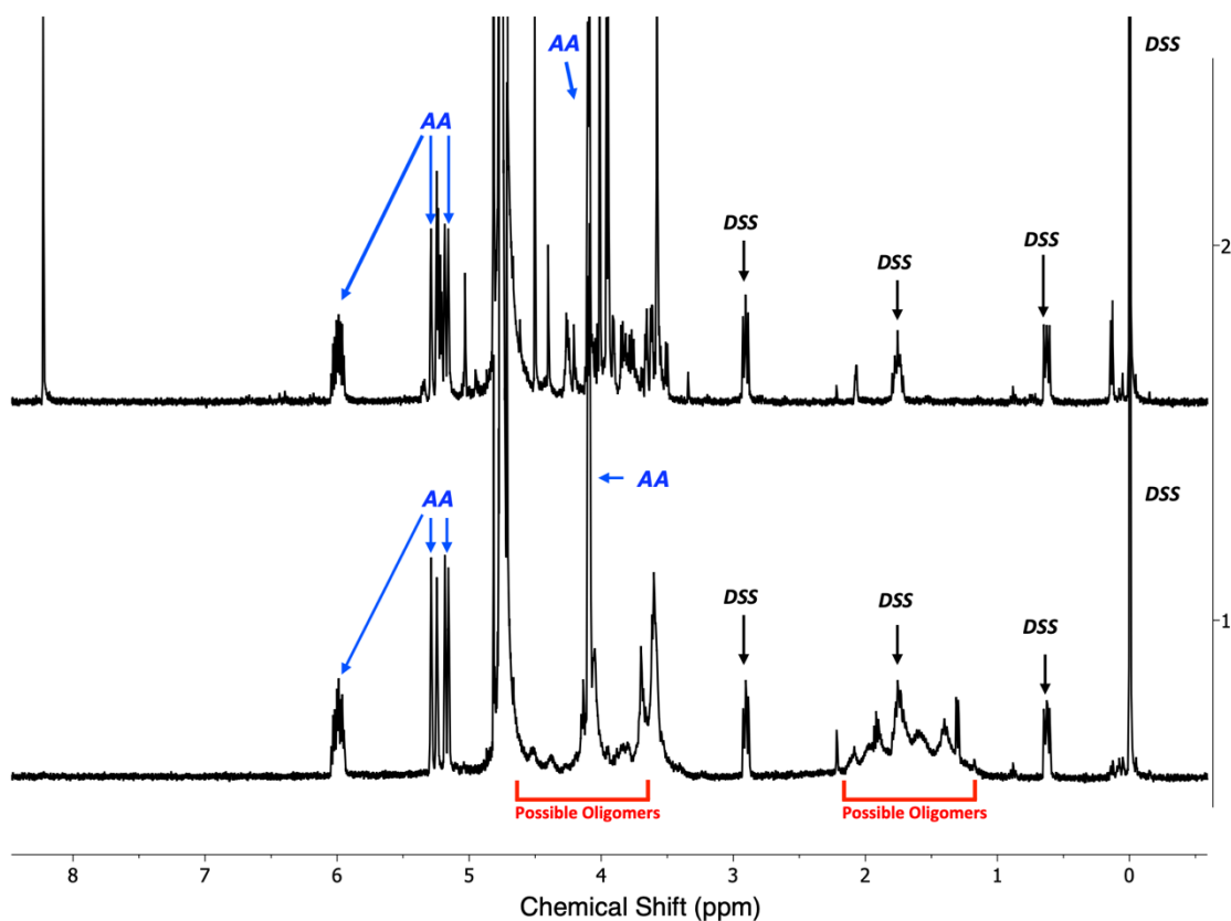
Figure 1. An ^1\text{H} -NMR spectrum of the oxygen saturated AA experiment (after 60 minutes of irradiation) (top) compared to an ^1\text{H} -NMR spectrum of the low oxygen AA experiment (after 45 minutes of irradiation) (bottom). The broad peaks (due to the presence of a large number of chemically similar but structurally unique protons) in the low oxygen experiment indicates the presence of oligomers.
