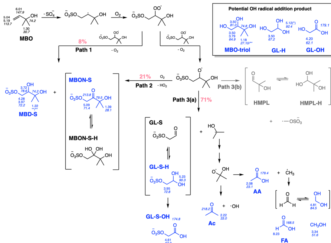
Figure 3. Proposed mechanism for the sulfate radical addition to MBO. Observed products (with their ^1\text{H} and/or ^{13}\text{C} NMR chemical shifts indicated) are labelled in blue, while unobserved pathways are labelled in grey. The branching ratios of the photochemical experiment are listed for each leg of reaction in pink.
