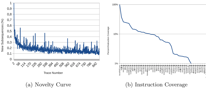
Fig. 6. The percentage of new subsequences appearing in each subsequent trace (left) and the coverage of instructions by library (right) for the Acrobat Reader dataset. Note that we do not expect full coverage of third-party libraries.
