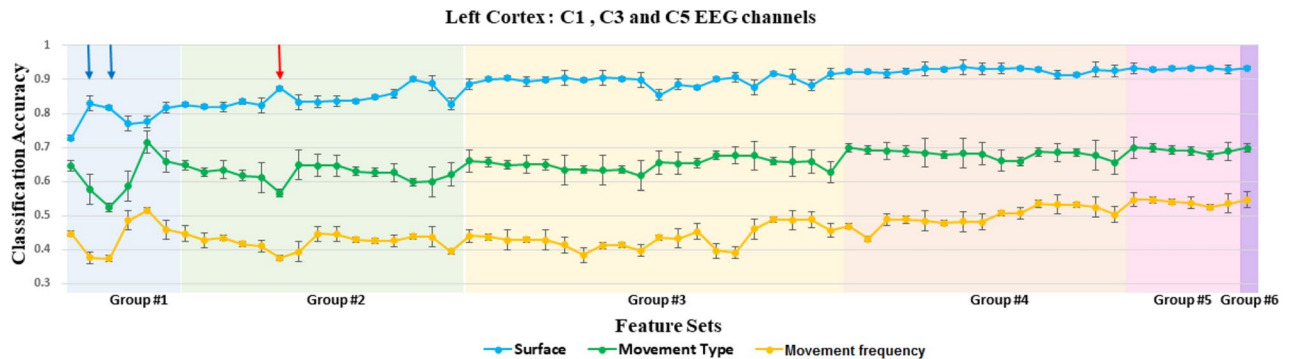
Figure 1. The mean and standard deviation of the classification accuracy of each classification problem (texture, movement type and frequency) calculated at each feature set and averaged across all the participants and all conditions and averaged over the three EEG channels (C1, C3 and C5). Each group of feature sets is highlighted by different background color. The selected set of features are marked by the blue and red arrows.
