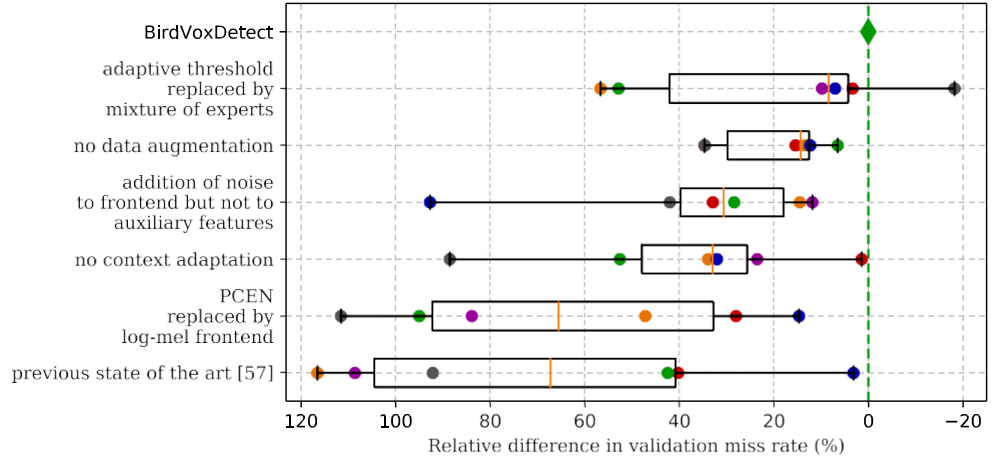
Fig 6. Ablation study of best model (CNN+PCEN+CA+GDA) on the BirdVox-full-night dataset. Boxes (resp. whiskers) denote interquartile (resp. extremal) variations between sensors.
