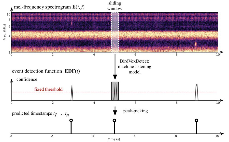
Fig 2. Overview of the presented baseline. After training a deep learning model to identify the presence of a sound event within short audio clips (150 ms), we run this model on a continuous recording by a sliding window procedure. We compare the peaks in the resulting event detection function (EDF) with a fixed threshold \tau in order to obtain a list of predicted timestamps for the sound event of interest. In the case of the presented baseline, these sound events of interest are avian flight calls; the input representation is a mel-frequency spectrogram; and the deep learning model is a convolutional network.
