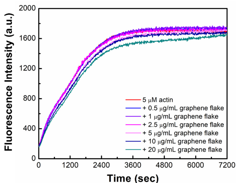
Figure 1. Graphene flakes do not hamper bulk actin polymerization. Actin (5 \mu M, 20% pyrene-labeled) polymerization in the presence of graphene flakes at varying concentrations (0.5–20 \mu g/mL) was monitored. Data are a representative from triplicated trials.
