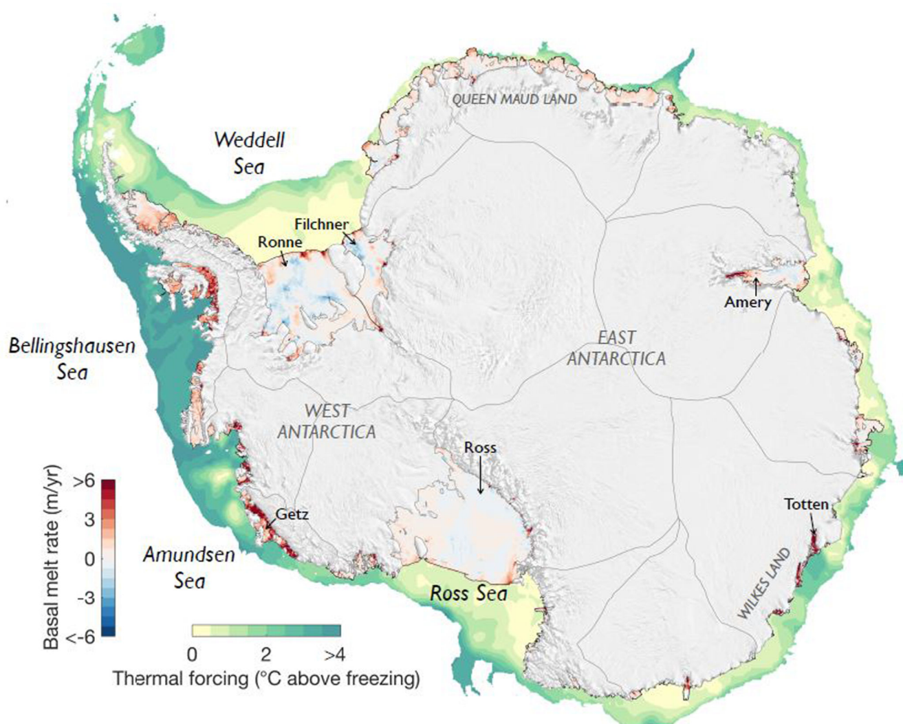
Figure 1: Basal melt rates of Antarctic ice shelves using CryoSat-2 altimetry. Rates are averaged over 2010–2018 and shown at 500 m posting. The units are m of ice equivalent, assuming an ice density of 917 \text{ kg/m}^3 . The thermal forcing, defined as the temperature above the in situ freezing point of seawater, is mapped for water depths <1500 m. For water depths less than 200 m the seafloor thermal forcing is shown, and for water depths >200 m, the maximum thermal forcing between 200 m and 800 m is shown (Methods Section S2).
