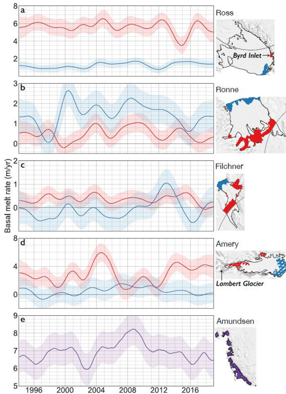
Figure 4: Time-dependent basal melt rates for different modes of melting.
