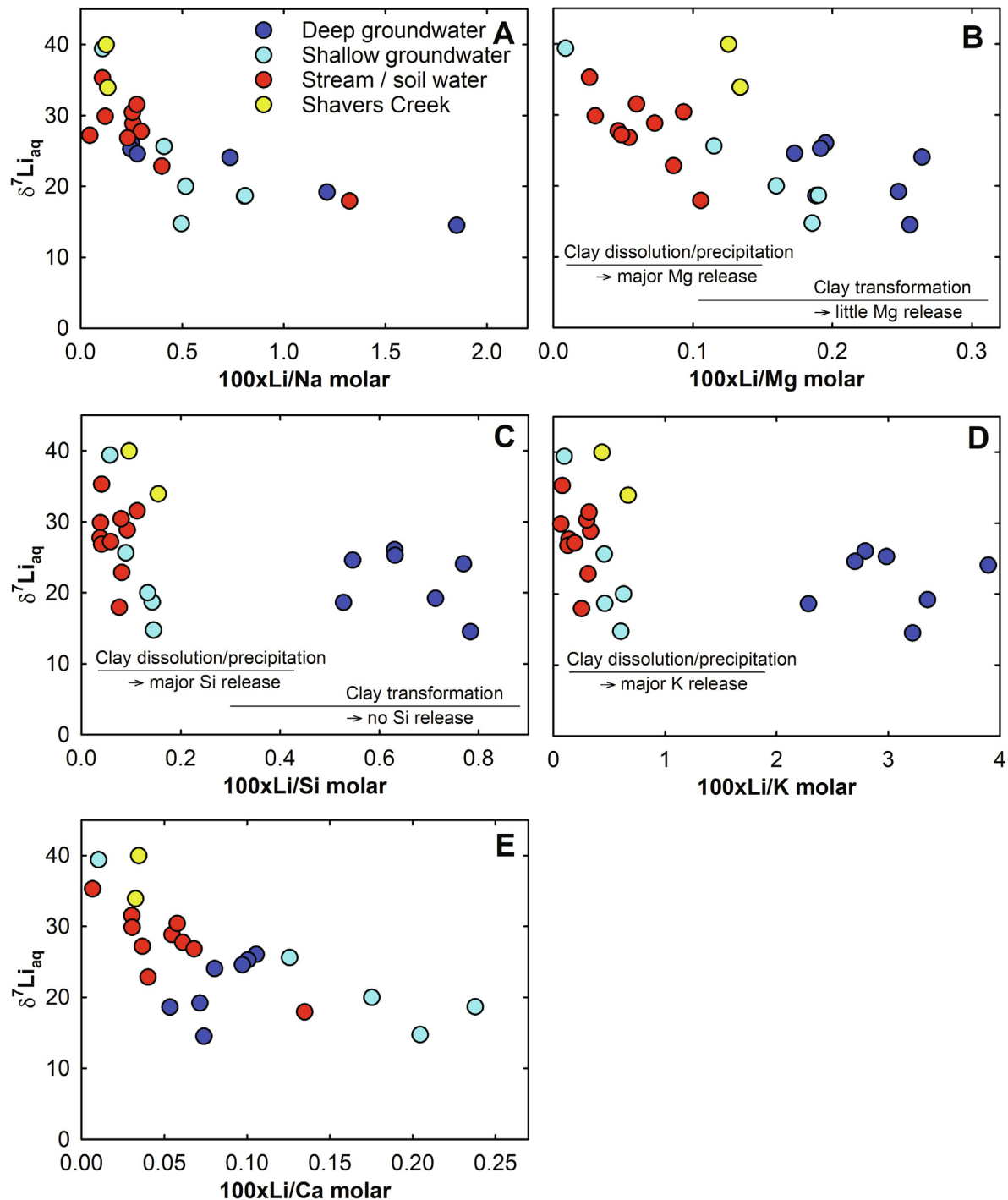
Fig. 6. Lithium isotopic composition of water samples versus Li/element ratio (mol:mol).
