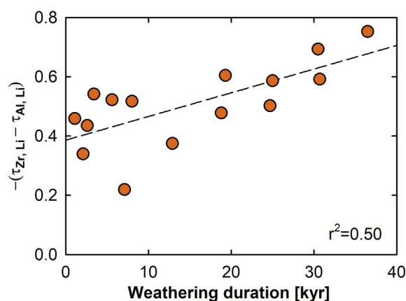
Fig. 11. Fractional depletion of Li from soils by the process of subsurface particulate transport -(\tau_{Zr,Li} - \tau_{Al,Li}) plotted versus weathering duration. Lithium depletion in soils by particle export correlates with weathering duration obtained by U-series (Ma et al., 2013). This plot indicates that about 40% of Li has been already lost by particles at zero duration of weathering, i.e., particulates are lost in the subsurface below the soil zone.
