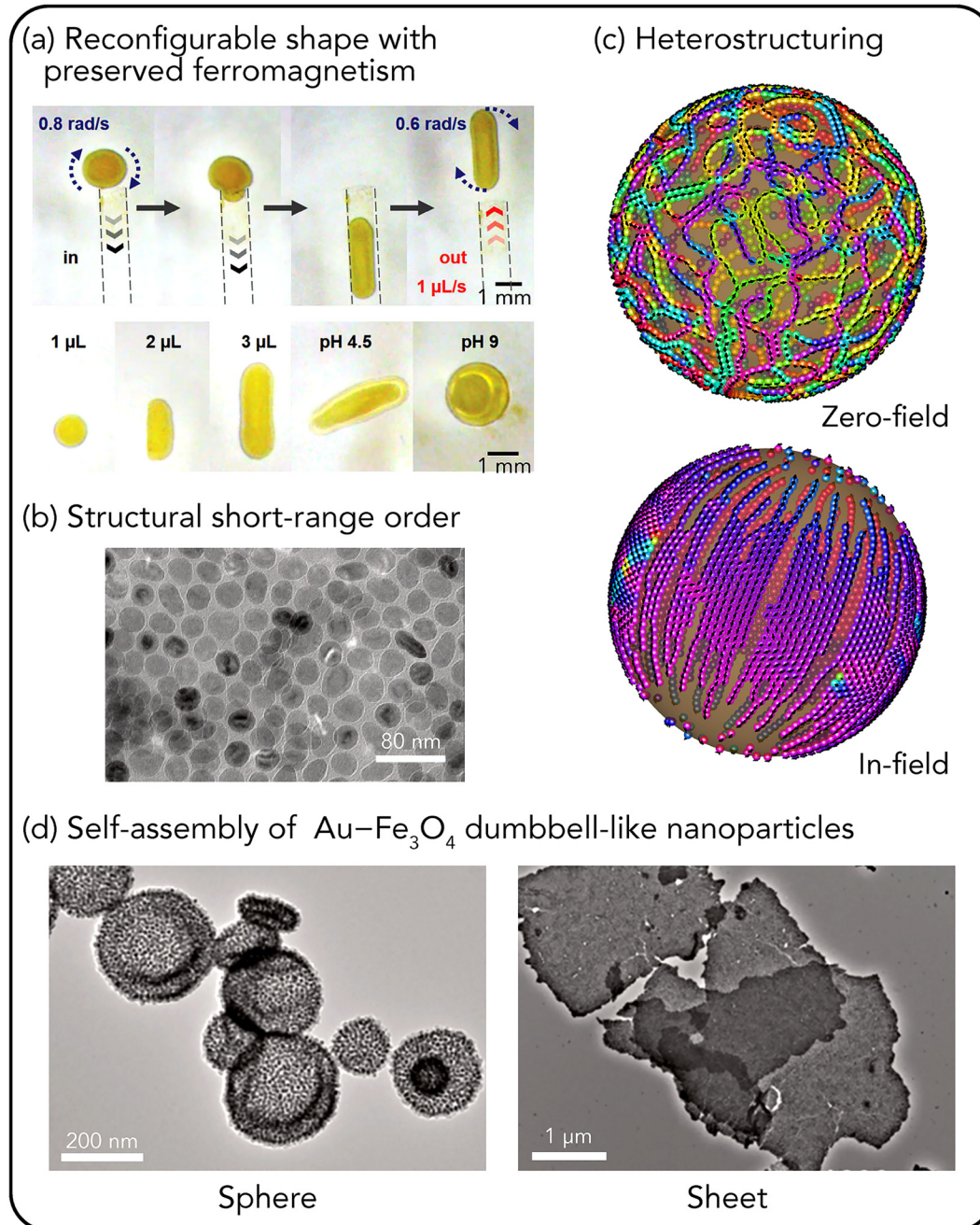
FIG. 10. Self-assembly of nanoparticle building blocks into 3D hierarchical systems in liquid environment. (a) Interfacial jamming of superparamagnetic nanoparticles at liquid–liquid interfaces forming ferromagnetic liquid droplets with reconfigurable shape and preserved magnetization observed in hydrodynamics experiments. Reproduced with permission from Liu et al. , Science 365 , 264 (2019). Copyright 2019 American Association for the Advancement of Science. (b) Isotropic elastic and magnetic properties stemming from structural short-range order of jammed nanoparticles imaged with transmission electron microscopy in their dried state. Reproduced with permission from Wu et al. , Proc. Natl. Acad. Sci. U.S.A. 118 , e2017355118 (2021). Copyright 2021 National Academy of Sciences. (c) In-field and zero-field assembly of nanoparticles from a mixture of dispersed superparamagnetic and non-magnetic nanoparticles revealing distinct heterostructures with enhanced magnetic anisotropy and remanent magnetization. The depicted states are modeled with molecular dynamics and micromagnetic simulations and leave out non-magnetic nanoparticles. (d) Self-assembly of \text{Au-Fe}_3\text{O}_4 dumbbell-like nanoparticles with packing parameter of (left) 0.63 and (right) 0.84 visualized with transmission electron microscopy. Reproduced with permission from Liu et al. , Nano Lett. 20 , 8773 (2020). Copyright 2020 American Chemical Society.
