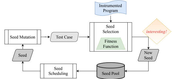
Fig. 1: Overview of greybox fuzzing
