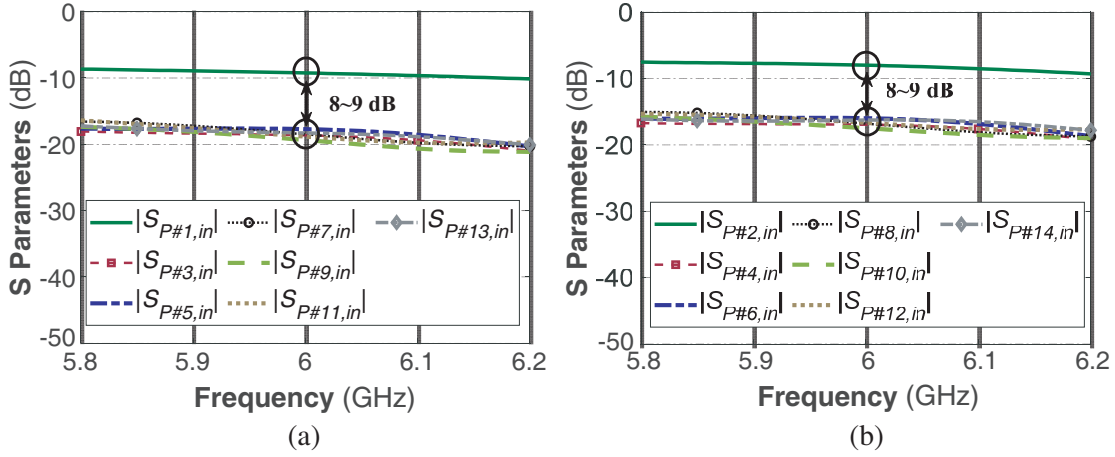
Figure 3. Simulated S -parameters representing amplitude tapering between (a) central elements ( p\#1 : TM 11 ) to peripheral elements TM 11 ports, (b) central elements ( p\#2 : TM 21 ) to peripheral elements TM 21 ports.
