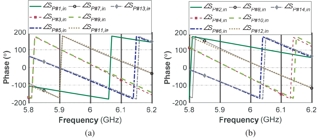
Figure 4. Simulated phase response of the (a) TM 11 , (b) TM 21 ports of the feeding network.
